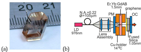
Fig. 1. (a) Photo of the as-grown Er,Yb:GdAB crystal; (b) scheme of the compact diode-pumped graphene PQS Er,Yb:GdAB laser: LD – laser diode, PM – pump mirror, OC – output coupler.
