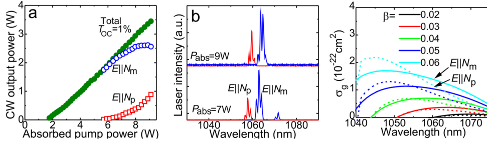
Fig. 5. Evidence of polarization-switching in the Yb:KLuW microchip laser at low inversion levels. (a) Output vs. absorbed pump power (filled symbols: total output, open symbols: contributions of E \parallel N_m and E \parallel N_p ); (b) laser spectra – simultaneous emission of both polarizations; (c) anisotropy of gain cross-sections, \sigma_g , for inversion ratios \beta \leq 0.06 .
