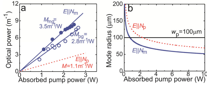
Fig. 3. (a) Optical power of the thermal lens in Yb:KLuW for light polarizations \mathbf{E} \parallel N_m (symbols: experimental data, solid lines: linear-fits) and \mathbf{E} \parallel N_p (dashed line, calculation); (b) calculated radius of the intracavity mode of the Yb:KLuW microchip laser.
