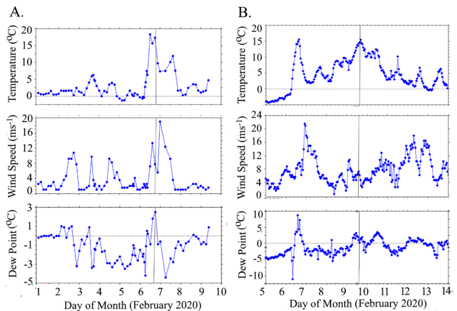
Fig. 2. Meteorograms of (top) temperatures ( ^\circ\text{C} ), (middle) wind speeds ( \text{m s}^{-1} ), and (bottom) dew points ( ^\circ\text{C} ) for (a) Esperanza station (Argentina) and (b) Marambio station (Argentina) on Seymour Island (located near the Brazilian permafrost monitoring station, see Fig. 1) for selected days in February 2020. The plots in (a) and (b) are constructed so they are each centered about the specific days under investigation (6 Feb, Esperanza; 9 Feb, Seymour Island). The thin black lines at 1500 UTC (1200 LST) 6 Feb 2020 in (a) and 1500 UTC (1200 LST) 9 Feb 2020 in (b) indicate times of the specific observations under investigation.
