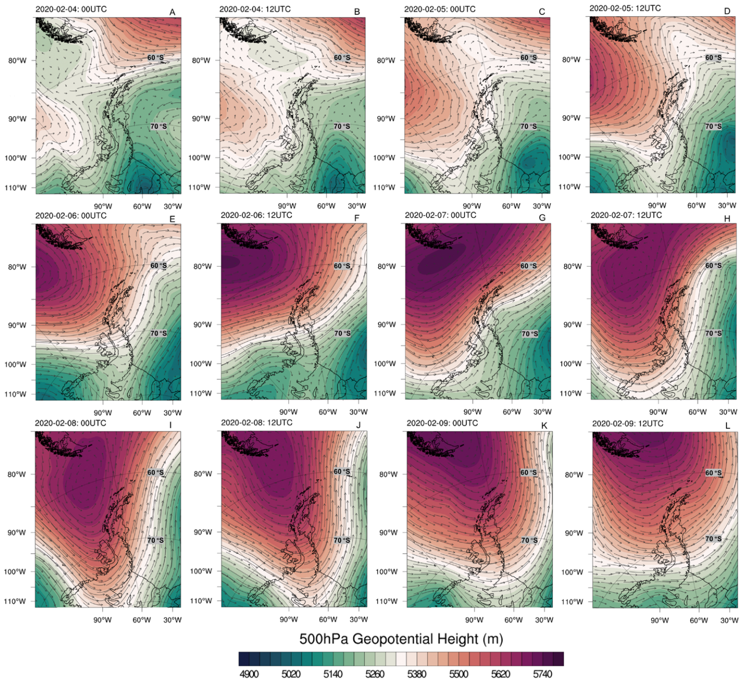
Fig. 3. ERA5 reanalysis regional 500-hPa heights (geopotential meters) together with 500-hPa vector winds for the Antarctic region for the period from (a) 0000 UTC 4 to (l) 1200 UTC 9 Feb 2020. The Esperanza 18.3°C data point occurred at approximately 1500 UTC 6 Feb 2020. The Seymour Island permafrost monitoring site 20.8°C data point occurred at approximately 1500 UTC 9 Feb 2020.
