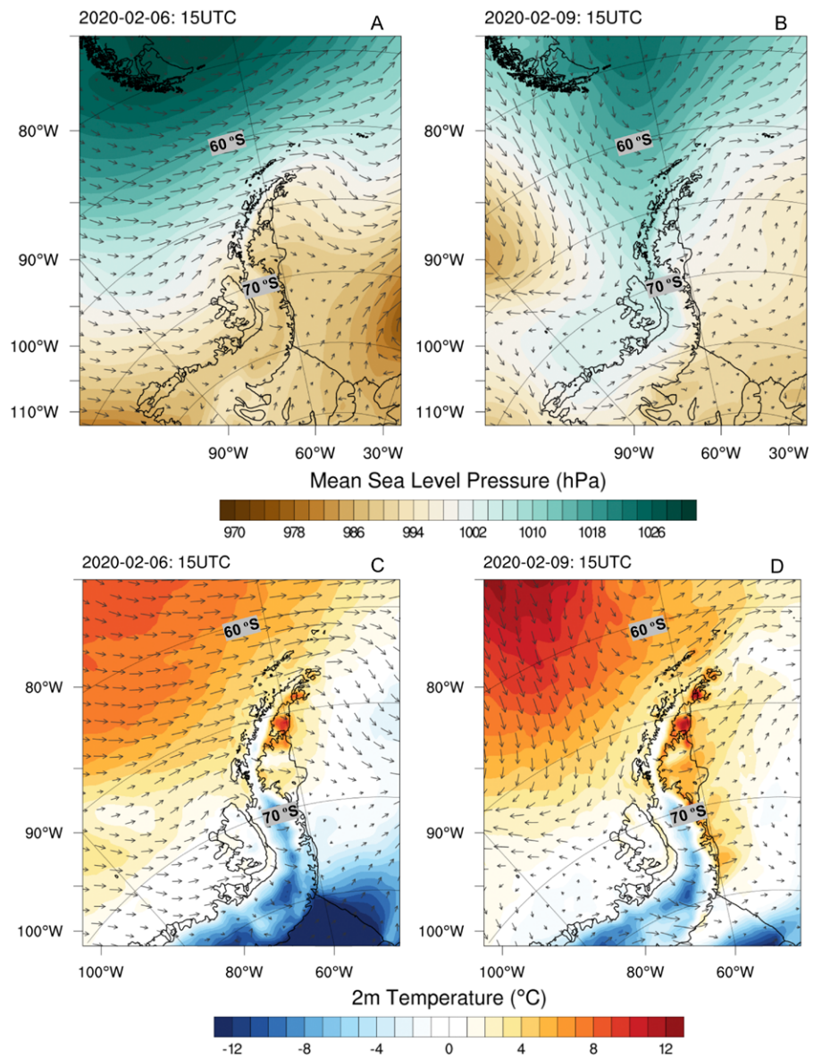
Fig. 4. ERA5 reanalysis mean sea level pressure (hPa) with 10-m vector winds for (a) the Esperanza 18.3^\circ\text{C} (1500 UTC 6 Feb 2020) and (b) the Seymour Island permafrost monitoring site 20.8^\circ\text{C} (1500 UTC 9 Feb 2020). ERA5 reanalysis of Antarctic Peninsula for 10-m vector winds and 2-m temperatures (c) for the Esperanza event and (d) for the Seymour Island permafrost monitoring event.
