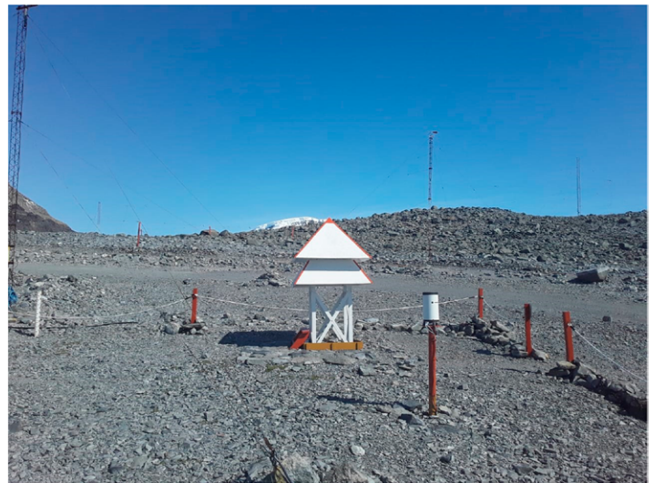
Fig. 5. Site photograph of temperature sensor at Esperanza station, looking to the south-southwest. Photograph by Sergio Fabián Montoya, taken in February 2020.
