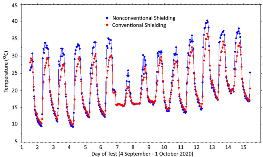
Fig. 7. Brazilian mountain test site comparison of hourly temperatures (°C) between conventional and nonconventional (i.e., the Seymour Island permafrost monitoring station) Campbell 107 sensor protection shields. The test was conducted from 4 Sep to 1 Oct 2020, days 1–6 (4–9 Sep), days 7–15 (22 Sep–1 Oct).
