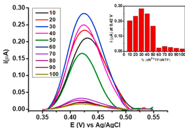
Fig. 3. Solid-phase RPA with all four dN FC TPs. SWV after SP-RPA using all four dN FC TPs/dNTPs at different percentages. The peak intensities vs. % dN FC TPs/dNTPs are shown in the inset.
