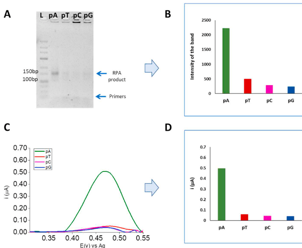
Fig. 4. SNP detection in a dsDNA target containing SNP T, prepared from synthetic ssDNA (Table S18), (pA - primer A-pT; primer T; pC- primer C; pG-primer G: L -Ladder). (A) Electrophoresis gel of RPA products amplified in solution; (B) corresponding intensities of the electrophoresis gel calculated by Image J software; (C) SWV of solid-phase approach and (D) The peak intensities of SWV of solid-phase approach. In all cases using 30% all four dN Fc TP/dNTP at the optimum conditions.
