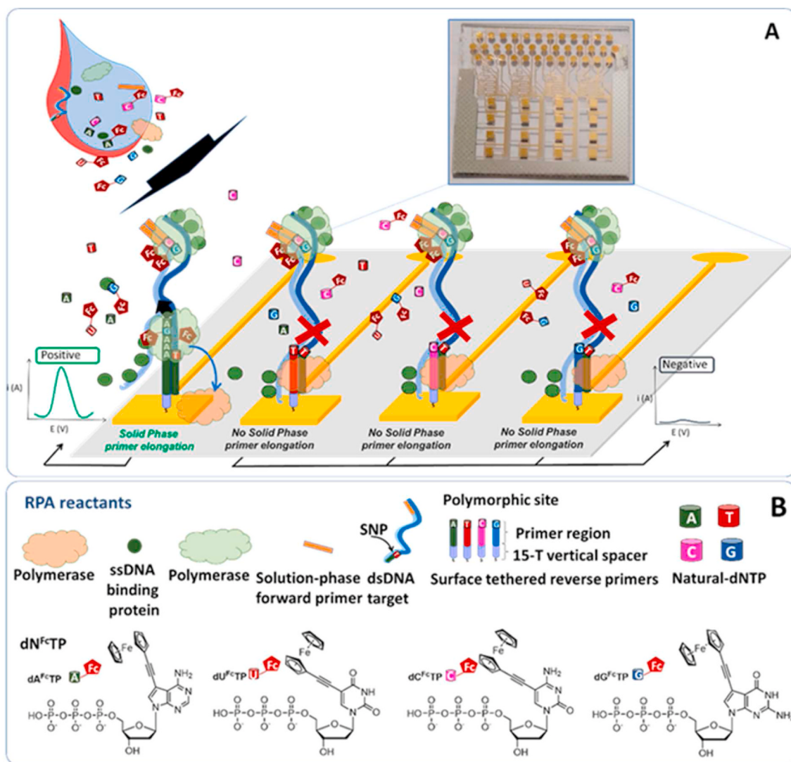
Fig. 1. (A) Schematic representation of the solid phase-RPA reaction carried out for SNP detection (Photograph of the actual electrode array in the inset). A detailed flow-through of the assay is shown in SM (Fig. S1) while magnified and detailed photographs of electrode array and microfluidics are shown in SM (Fig. S2); (B) RPA reagents and structure of ferrocene labelled dNTPs (dN Fc TP) used for the reaction.
