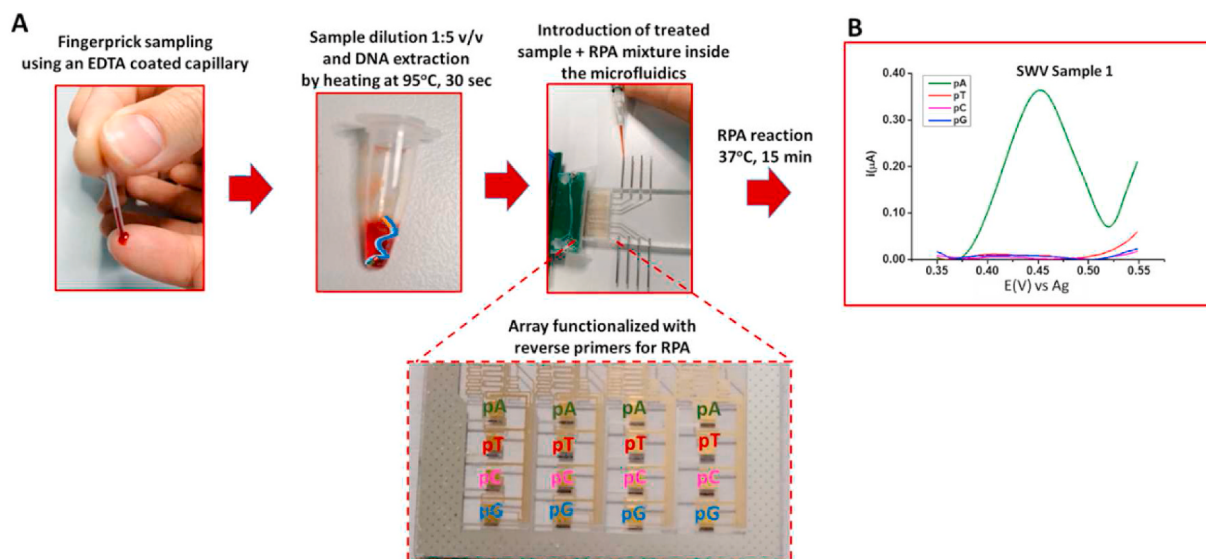
Fig. 5. SNP detection in real samples. (A) Flow through of SNP detection using fingerprick samples (pA - primer A-pT; primer T; pC- primer C; pG-primer G) and (B) SWV of RPA product amplified from a fingerprick blood sample.
