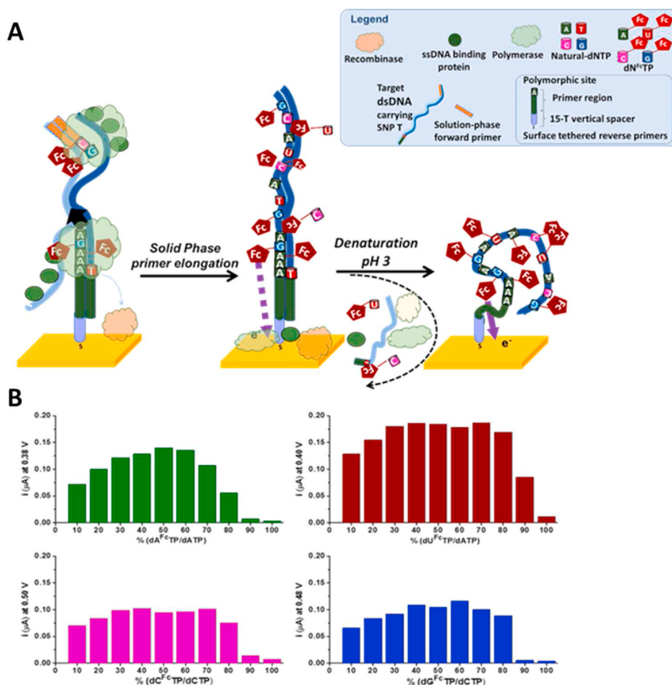
Fig. 2. (A) Schematic representation of the solid-phase RPA reaction, including the potential non-specific intercalation of dN Fc TP in the double helix of amplified product and non-specific adsorption of the RPA proteins on the surface of electrode, which are effectively removed via the addition of the glycine-HCl, pH 3; (B) SWV peak intensities after SP-RPA using individual dN Fc TP/dNTP at different percentages.
