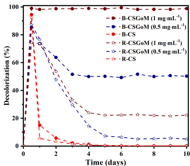
Fig. 8. Decolorization of AO7 in CS and CSGoM reactors; CS and CSGoM bioreactors; Flux = 0.05 \text{ L} \cdot \text{m}^{-2} \cdot \text{h}^{-1} , AO7 concentration in feed solution = 50 \text{ mg} \cdot \text{L}^{-1} and T = 37^\circ \text{C} . (For interpretation of the references to color in this figure, the reader is referred to the web version of this article.)
