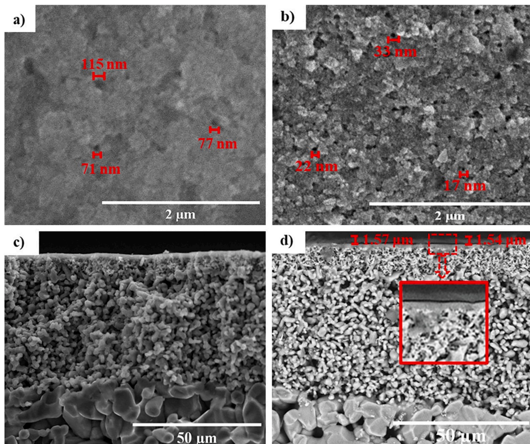
Fig. 5. FESEM micrographs on the surface of a) CS and b) CSGoM-1, and the cross section of c) CS and d) CSGoM-1 (deposited GO amounts: 2.6 mg).
