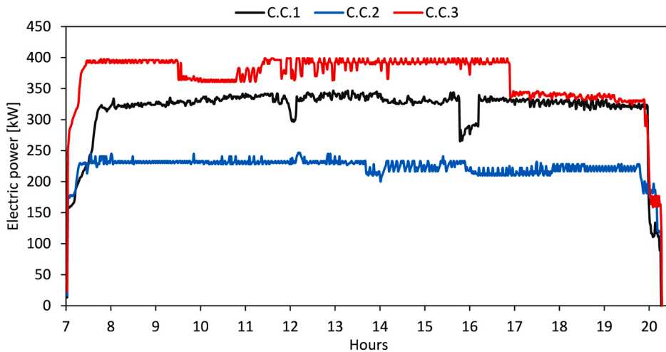
Fig. 5. Power demand from mechanical vapour compression chillers.
