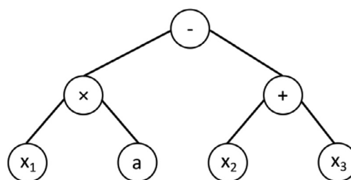
Fig. 1. Representation of the equation f(x_1, x_2, x_3) = ax_1 - (x_2 + x_3) using a binary tree.
