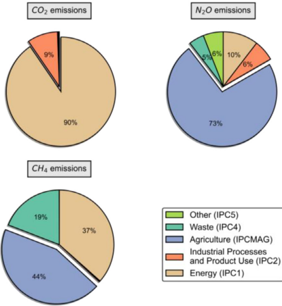
Fig. 3. Source of the greenhouse gas (GHG) emissions per sector in 2018 from PRIMAP-hist (Gütschow et al., 2016).
