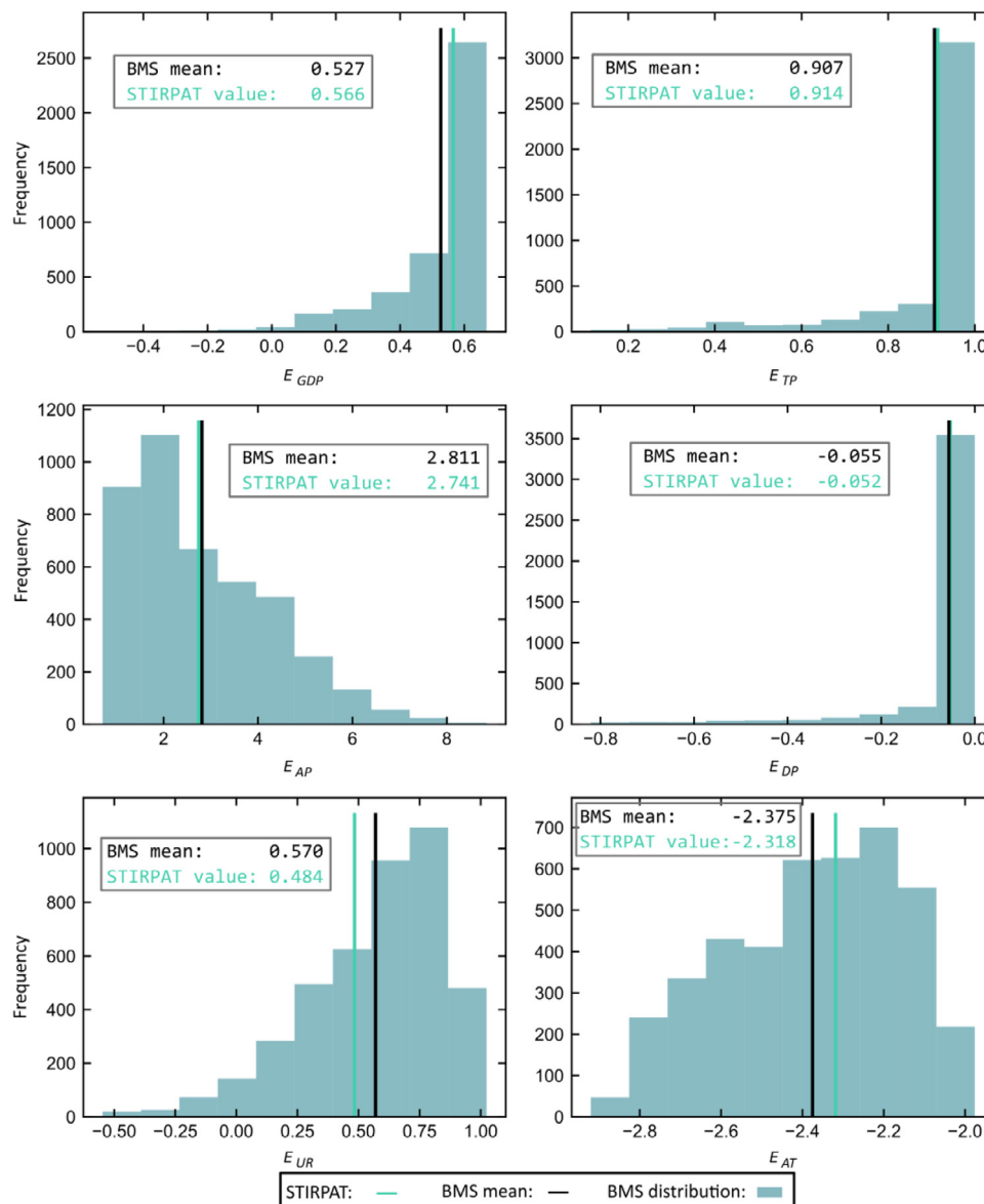
Fig. 5. Elasticities of models of CO 2 emissions. E_x refers to the elasticity with respect to driver x , where x = GDP, TP (total population), AP (active population), DP (density of population), UR (urbanization rate), and AT (average temperature). The histogram shows the distribution of the elasticities obtained from the Bayesian Machine Scientist (BMS) model for each data point. Vertical lines correspond to the STIRPAT elasticity (turquoise) and the mean elasticity obtained from the BMS elasticity distribution (black).
