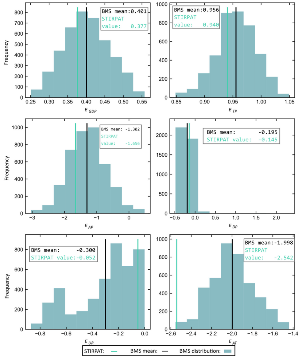
Fig. 7. Elasticities of the models of N_2O emissions. E_x refers to the elasticity with respect to driver x , where x = GDP, TP (total population), AP (active population), DP (density of population), UR (urbanization rate), and AT (average temperature). The histogram shows the distribution of the elasticities obtained from the Bayesian Machine Scientist (BMS) model for each data point. Vertical lines correspond to the STIRPAT elasticity (turquoise) and the mean elasticity obtained from the BMS elasticity distribution (black).
