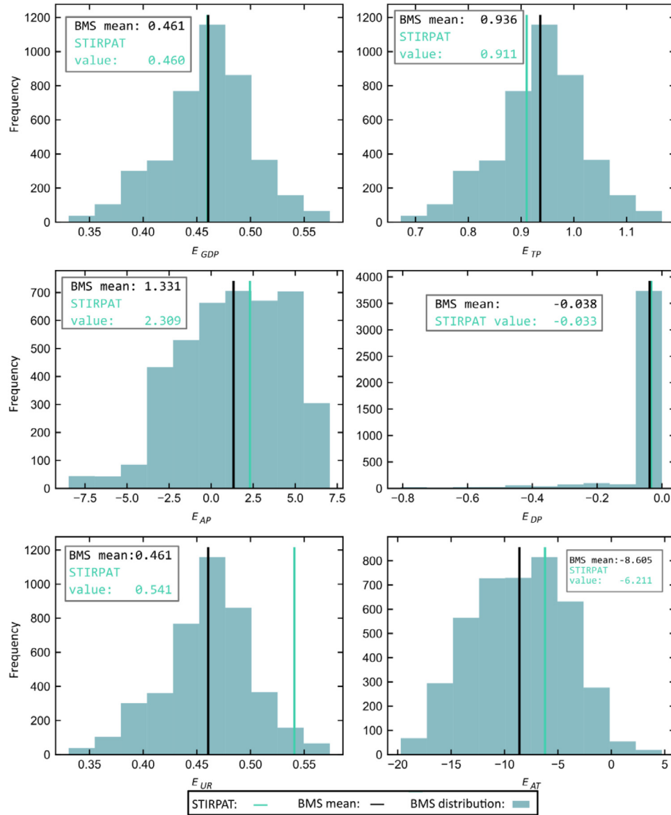
Fig. 6. Elasticities of the models of energy consumption. E_x refers to the elasticity with respect to driver x , where x = GDP, TP (total population), AP (active population), DP (density of population), UR (urbanization rate), and AT (average temperature). The histogram shows the distribution of the elasticities obtained from the Bayesian Machine Scientist (BMS) model for each data point. Vertical lines correspond to the STIRPAT elasticity (turquoise) and the mean elasticity obtained from the BMS elasticity distribution (black).
