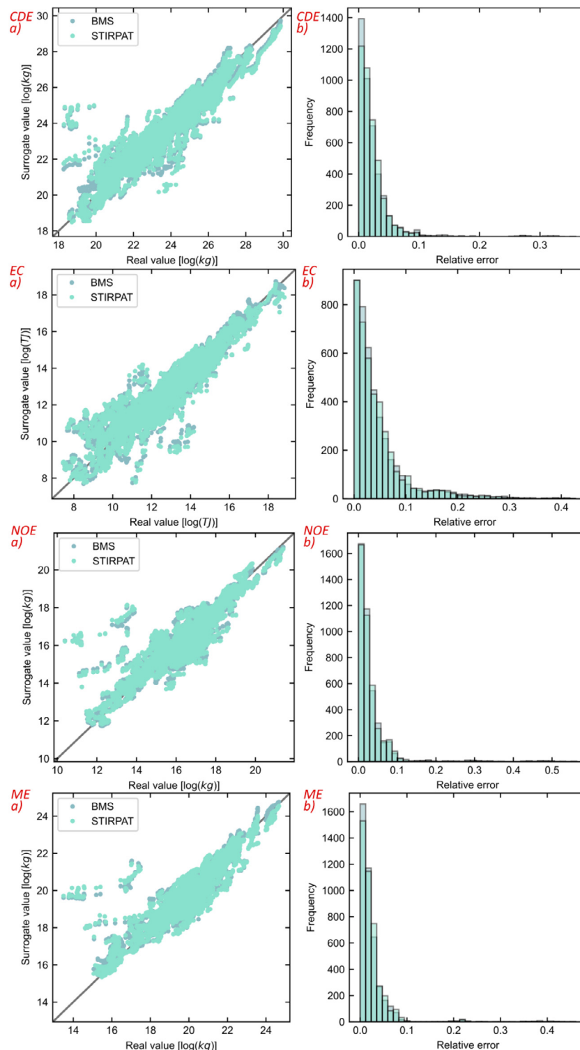
Fig. 4. Full data results for the four environmental impacts: a) Predicted value vs. real value, b) histogram of absolute relative errors for the STIRPAT and the Bayesian Machine Scientist (BMS) in the logarithmic space. The notation for the impact categories is as follows: CDE refers to CO 2 emissions, EC refers to energy consumption, NOE refers to N 2 O emissions and ME refers to methane emissions.
