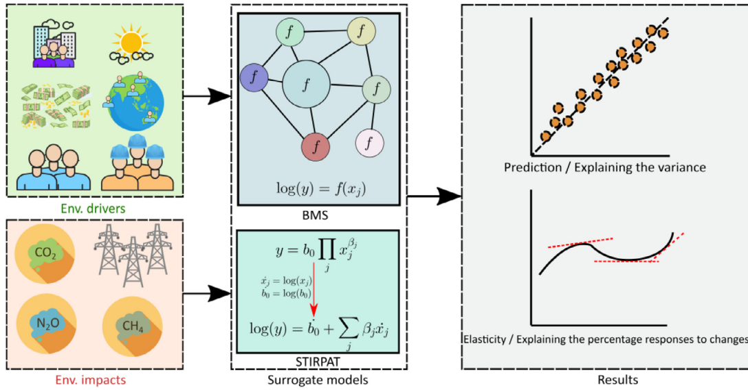
Fig. 2. Schematic representation of the methodology. We obtained two models for each impact using the Bayesian Machine Scientist (BMS) and the STIRPAT. For each of them, we compute a set of fitness metrics and the elasticities of the drivers.
