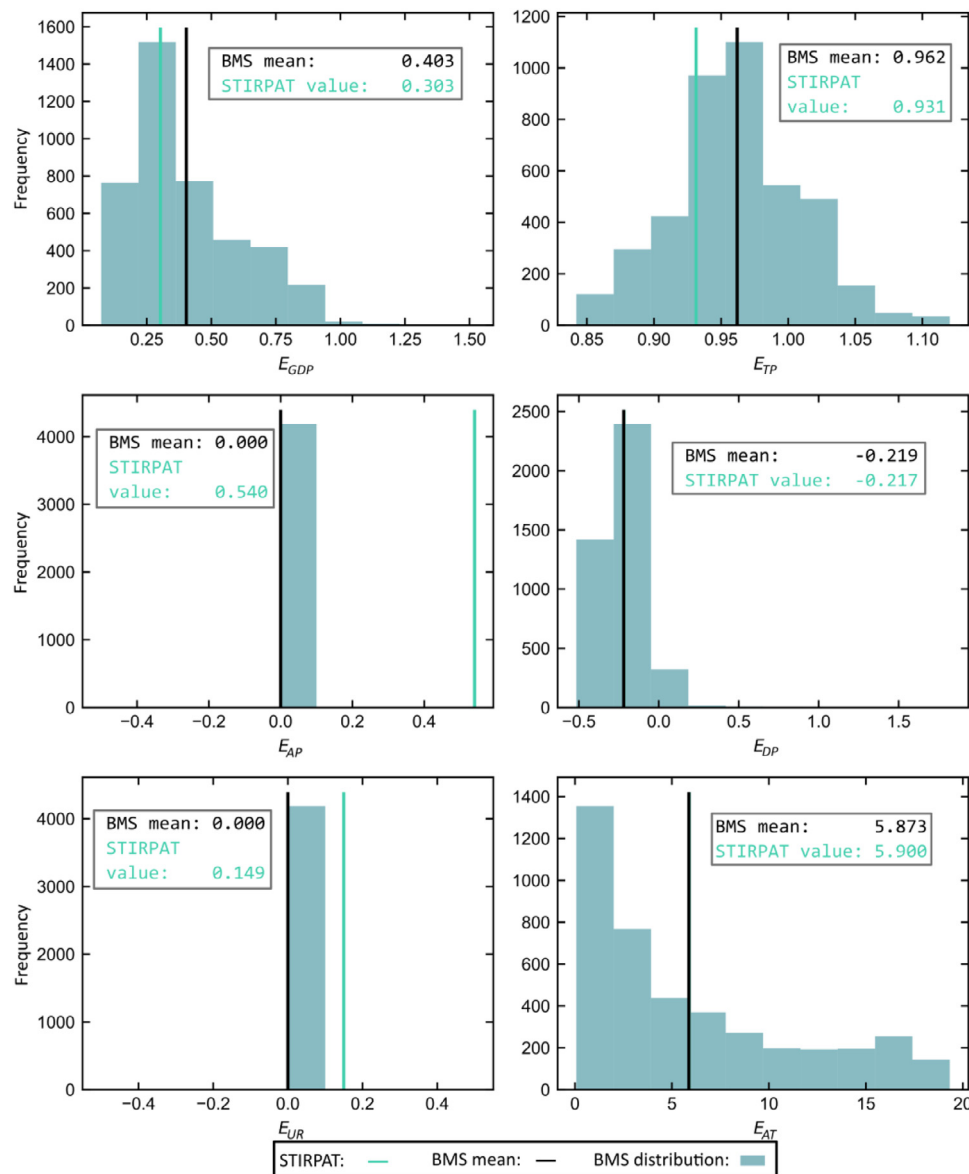
Fig. 8. Elasticities of the models of \text{CH}_4 emissions. E_x refers to the elasticity with respect to driver x , where x = \text{GDP} , TP (total population), AP (active population), DP (density of population), UR (urbanization rate), and AT (average temperature). The histogram shows the distribution of the elasticities obtained from the Bayesian Machine Scientist (BMS) model for each data point. Vertical lines correspond to the STIRPAT elasticity (turquoise) and the mean elasticity obtained from the BMS elasticity distribution (black).
