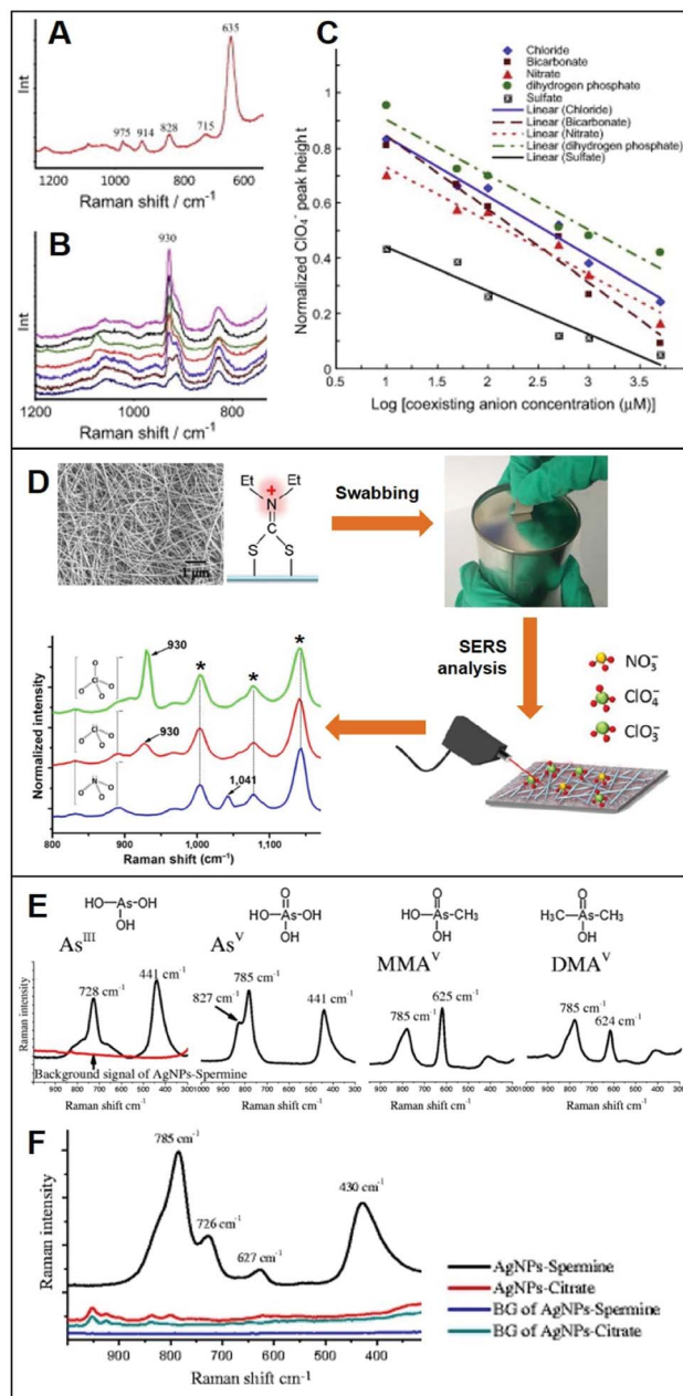
Fig. 4 Direct SERS detection of inorganic anions. (A) Background spectrum of the Cys on Ag nanofilm/Cu foil in deionized water. (B) SERS spectra of a 50 \mu\text{M} \text{ClO}_4^- solution in the presence of different concentrations of \text{HCO}_3^- (0, 10, 50, 100, 500, 1000 and 5000 \mu\text{M} , from top to bottom). (C) Normalized \text{ClO}_4^- peak height plotted against concentration of coexisting anions ( \text{Cl}^- , \text{NO}_3^- , \text{SO}_4^{2-} , \text{HCO}_3^- and \text{H}_2\text{PO}_4^- ) in logarithmic scale ( \log \mu\text{M} ). Adapted with permission from ref. 79 Copyright 2015, Elsevier. (D) SEM image of the Ag nanowire membrane and surface modification with diethyldithiocarbamate (DDTC) which is used as a swab to collect trace amounts of \text{ClO}_4^- , \text{ClO}_3^- and \text{NO}_3^- anions onto a surface. SERS analysis of the swabbed membrane onto surfaces with 2.0 \mu\text{g} of \text{ClO}_4^- , 1.7 \mu\text{g} of \text{ClO}_3^- and 1.2 \mu\text{g} of \text{NO}_3^- (asterisks: DDTC bands). Adapted with permission from ref. 80 Copyright 2016, Springer. (E) Individual SERS spectra of four arsenic species (4 ppm) on spermine-coated silver nanoparticles (AgSp). (F) SERS spectra of a mixture of the four arsenic species (200 ppb) in the cell lysate on negatively-charged citrate silver colloids (AgCit) and AgSp. The background signals AgCit and AgSp were also included. Adapted with permission from ref. 56 Copyright 2017, Springer.
