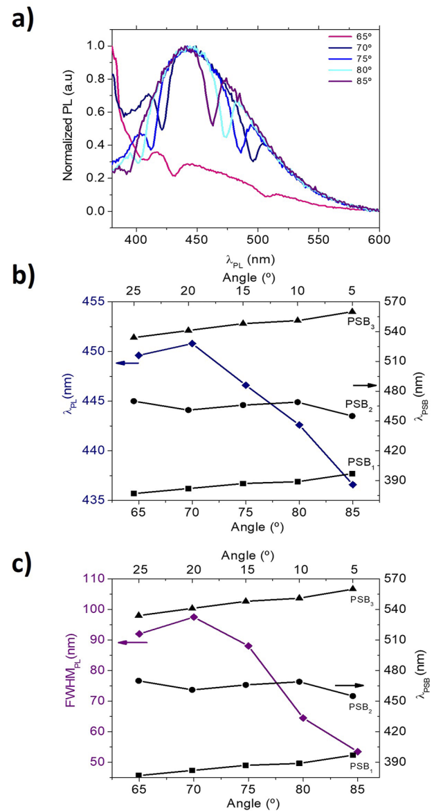
FIG. 7. Summary of the position of PSB 1 , PSB 2 , and PSB 3 and the features of PL emission from MS-NAA-PCs (NB: angles of reflection and emission were complementary at 25^\circ - \theta reflection + \theta emission = 90^\circ ). (a) PL emission from MS-NAA-PCs at 65^\circ , 70^\circ , 75^\circ , 80^\circ , and 85^\circ . (b) Dependence of \lambda_{PL} and the position of PSB 1 , PSB 2 , and PSB 3 in MS-NAA-PCs with the angle of incidence. (c) Dependence of FWHM_{PL} and the position of PSB 1 , PSB 2 and PSB 3 in MS-NAA-PCs with the angle of incidence.
