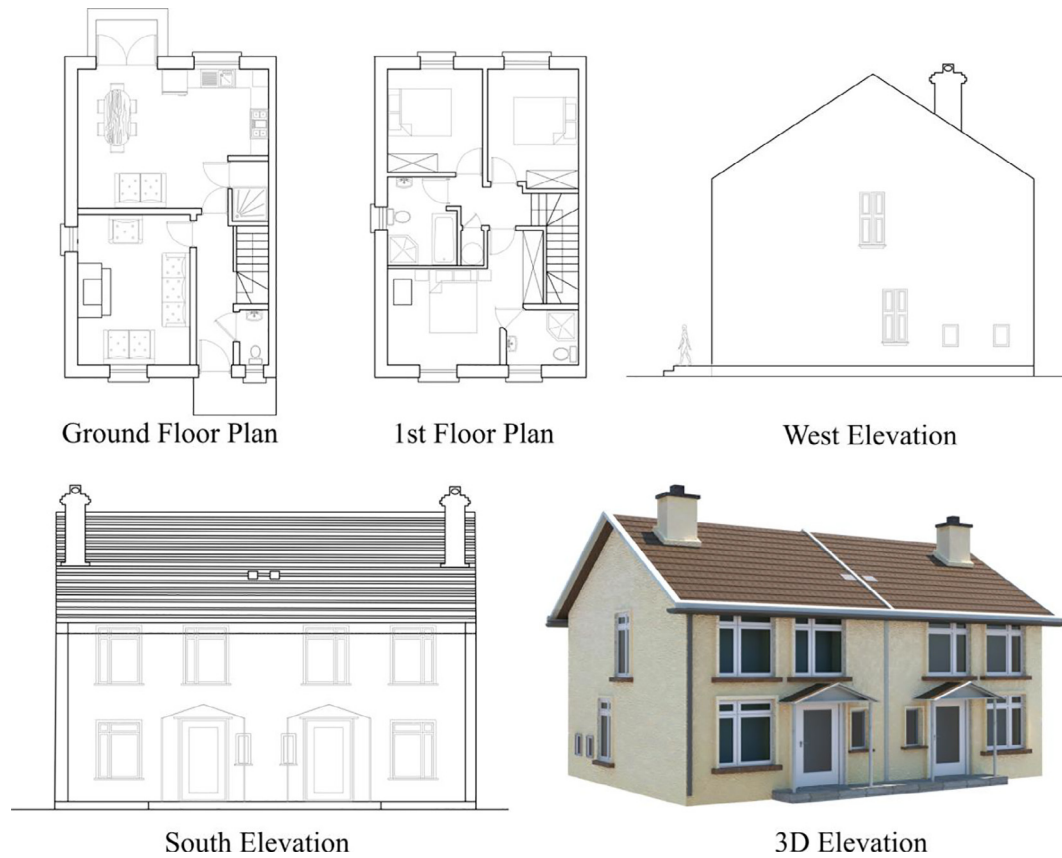
Fig. 4. 2D and 3D model of the reference house.
