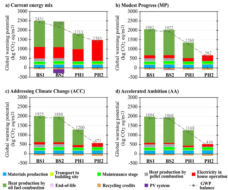
Fig. 8. Global warming potential associated with current energy mix and three future electricity mix scenarios for different case studies for the lifespan of 60 years.
