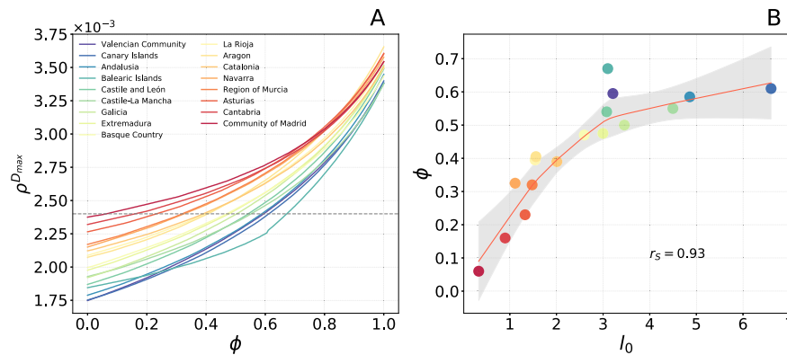
Fig. 4. Permeability, saturation of the health system & structural correlations. A. Maximum number of detected individuals during the first epidemic wave \rho_{max} as a function of the social permeability \phi allowed for each autonomous region. The dashed line indicates the threshold used, 2.4 \times 10^{-3} , to calculate the permeability that can be afforded by each territory. B. Correlation between the affordable permeability of each community \phi^{aff} and the average shortest contagion path connecting a random individual with the infection source in each territory l_0 . Solid red line shows the LOESS regression of the data whereas the shadowed region showed the 95% confidence interval obtained by bootstrapping 1000 samples.
