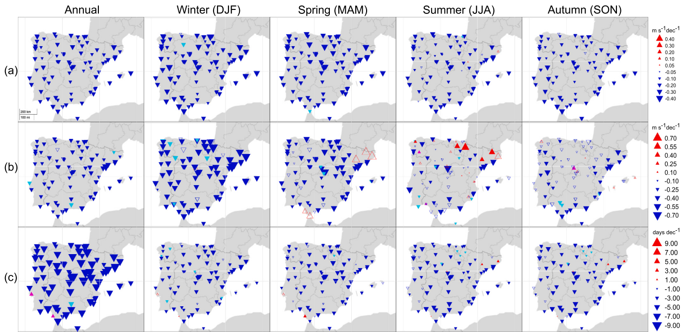
Fig. 5. Annual and seasonal spatial distribution of the sign, statistical significance and magnitude of trends of (a) monthly mean SWS anomaly (in \text{m s}^{-1} \text{dec}^{-1} ), (b) monthly mean DPWG anomaly (in \text{m s}^{-1} \text{dec}^{-1} ) and (c) f_{90}(\text{DPWG}) (in \text{days dec}^{-1} ) for the homogenized series of the 87 stations for 1961–2019. Blue and red filled triangles are significant at p < 0.05 ; cyan and magenta filled triangles are significant at p < 0.10 ; and non-filled triangles are non-significant at p < 0.10 . Different scales have been used for each variable in order to appreciate trends.
