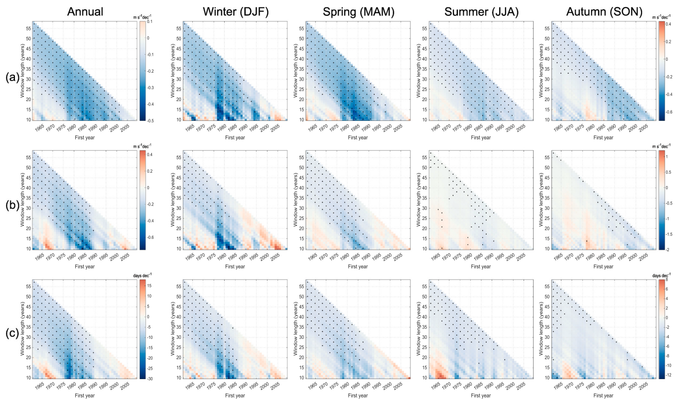
Fig. 4. Running trends analysis for (a) monthly mean SWS anomaly (in \text{ms}^{-1}\text{dec}^{-1} ), (b) monthly mean DPWG anomaly (in \text{ms}^{-1}\text{dec}^{-1} ) and (c) f_{90} (DPWG) (in \text{days dec}^{-1} ). X-axis indicates the starting year of any temporal window over which the trend is calculated and Y-axis represents the window length. Black dots indicate significant trends at p < 0.05 . Different scales have been used for each variable in order to appreciate trends.
