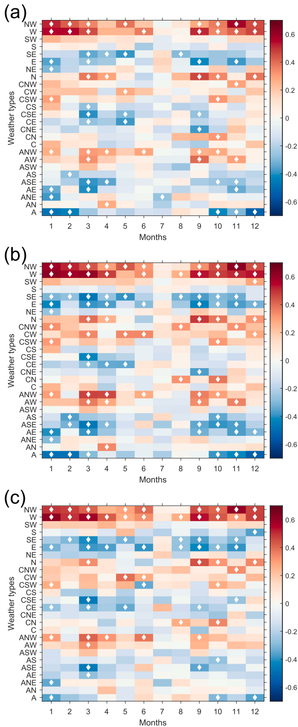
Fig. 9. Monthly Spearman's rank correlation coefficients between the 26 JC weather types and (a) monthly mean SWS anomaly, (b) monthly mean DPWG anomaly and (c) f_{90}(\text{DPWG}) for 1961–2019. White diamonds indicate significant correlation at p < 0.05 .
