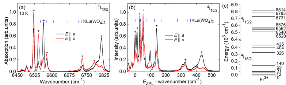
Fig. 9. (a,b) LT (10 K) (a) absorption and (b) luminescence spectra of \text{Er}^{3+} in the \text{MgWO}_4 crystal corresponding to the ^4\text{I}_{15/2} \leftrightarrow ^4\text{I}_{13/2} transition, “+” - assigned electronic transitions, dashes – electronic transitions for \text{Er}^{3+} in \text{KLu}(\text{WO}_4)_2 crystal [33]; (c) experimental Stark splitting of the ^4\text{I}_{15/2} and ^4\text{I}_{13/2} \text{Er}^{3+} multiplets, numbers indicate the sub-level energies in \text{cm}^{-1} .
