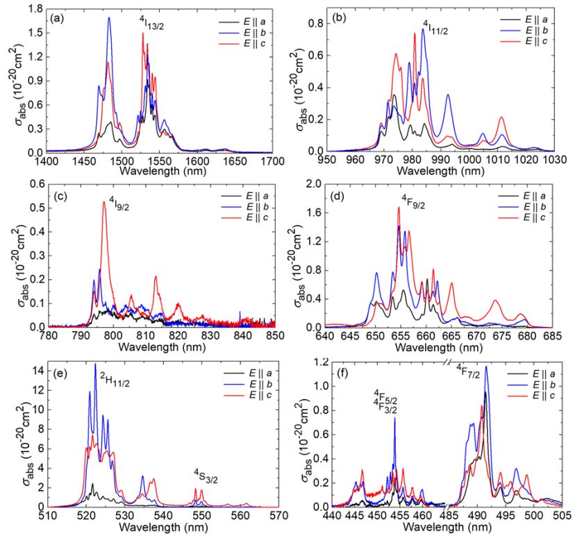
Fig. 4. (a-f) RT (293 K) absorption cross-section, \sigma_{\text{abs}} , spectra of \text{Er}^{3+}:\text{MgWO}_4 crystal, the light polarizations are E \parallel a, b, c .
