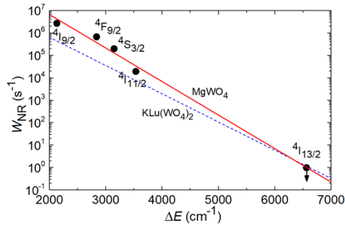
Fig. 8. The rate of multiphonon non-radiative relaxation W_{NR} vs. the energy gap to the lower-lying manifold \Delta E for \text{Er}^{3+} in \text{MgWO}_4 : circles – data obtained from luminescence lifetime measurements, red solid line – their fit, blue dashed line – fit for \text{KLu}(\text{WO}_4)_2 [31].
