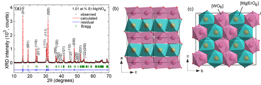
Fig. 2. Structural study of \text{Er}^{3+}:\text{MgWO}_4 : (a) X-ray powder diffraction (XRD) analysis: observed (black), calculated (red) and residual (blue) patterns, dashes – Bragg positions, (hkl) – Miller's indices; (b,c) projection of the crystal structure on (b) the a - c plane and (c) the b - c plane, black lines – unit-cell.
