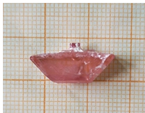
Fig. 1. A photograph of the as-grown 1.01 at.% \text{Er}^{3+}:\text{MgWO}_4 crystal, the growth direction is along the [010] axis.
