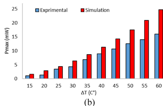
Fig. 9. Experimental versus simulation results: (a) Open circuit voltage, (b) Power max.
