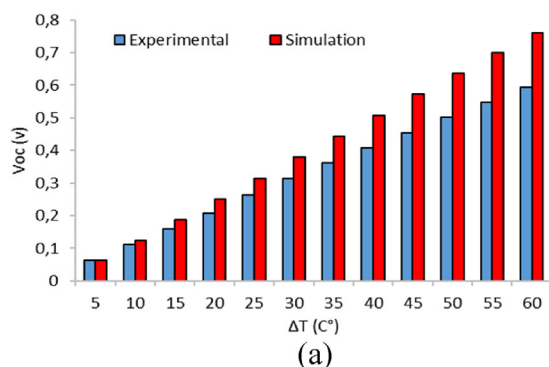
Fig. 9. Experimental versus simulation results: (a) Open circuit voltage, (b) Power max.
