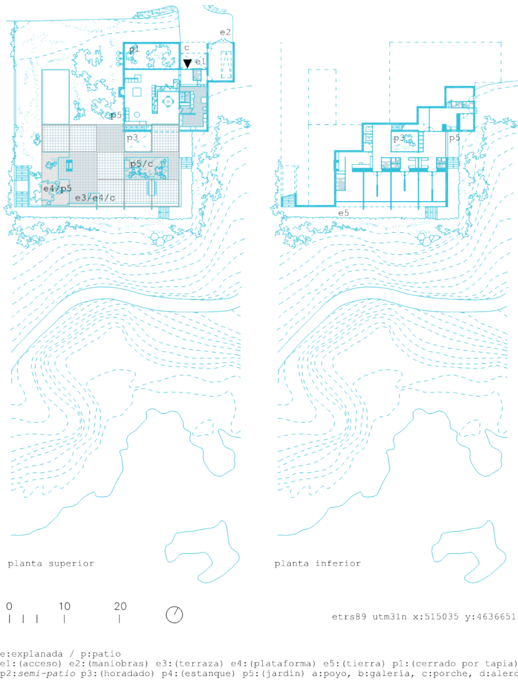
Figure 6. The Castanera house. Patios and esplanades.
