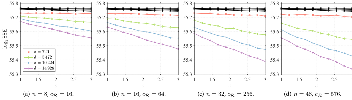
Fig. 9. Average distortion versus privacy protection for several values of record delay \delta , block size n and maximum allowed reordering cost c_R in the data set v1Census. The baseline approach and the proposed solution are represented with black and colored lines and points, respectively.
