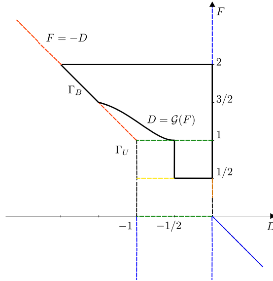
Fig. 1. The thick (closed) curve \Gamma_B consists of local bifurcation values of the period function at the outer boundary according to [23], where the curve that joins (-\frac{3}{2}, \frac{3}{2}) and (-\frac{1}{2}, 1) is the graphic of an analytic function D = \mathcal{G}(F) , see Remark 3.4. The dotted lines \Gamma_U correspond to parameters that remained unspecified in that paper and we color the subsequent improvements obtained in [19,24,25,27,28,38,39]. The parameters outside \Gamma_B \cup \Gamma_U are local regular values by the result in [23]. (For interpretation of the colors in the figure(s), the reader is referred to the web version of this article.)
