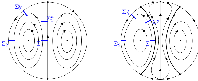
Fig. 5. Phase portrait of X_v for v = (D, F) \in (-1, 0) \times (0, +\infty) in the Poincaré disc with F \leq 1 (left) and F > 1 (right). In this case, contrary to the previous ones, the singularity at infinity for F = 1 is not a hyperbolic saddle but a saddle-node.
