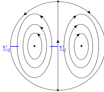
Fig. 3. Phase portrait in the Poincaré disc of X_v for v \in V , where for convenience the center at (0, 0) is shifted to the left and the vertical invariant line is \{x = 1\} .
