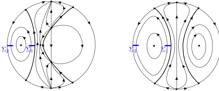
Fig. 4. Phase portrait in the Poincaré disc of X_\nu for \nu \in W with D < -1 (left) and D > -1 (right), where the center at (0, 0) is shifted to the left, the vertical invariant line is \{x = 1\} and the hyperbola \{\frac{1}{2}y^2 - q(x) = 0\} appears in boldface type.
