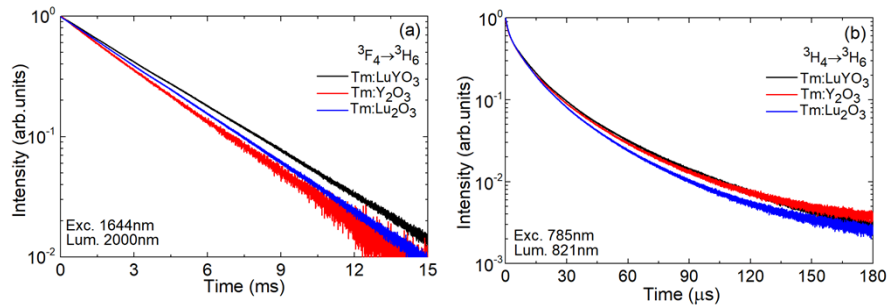
Fig. 8. RT luminescence decay curves for Tm^{3+} ions in the LuYO 3 , Y 2 O 3 , and Lu 2 O 3 ceramics: (a) decay from the ^3F_4 state, \lambda_{\text{exc}} = 1644 \text{ nm} , \lambda_{\text{lum}} = 2000 \text{ nm} ; (b) decay from the ^3H_4 state, \lambda_{\text{exc}} = 785 \text{ nm} , \lambda_{\text{lum}} = 821 \text{ nm} . Powdered samples.
