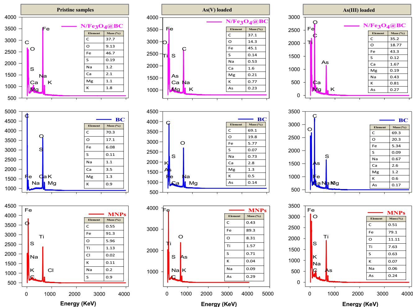
Fig. 2 EDS spectra of all tested adsorbent before and after As(III & V) adsorption.
