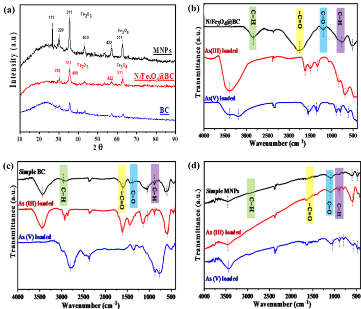
Fig 1. (a) XRD diffractogram and, (b–d) FTIR spectrum of all tested magnetite (N/Fe 3 O 4 @BC, BC, MNPs) before and after arsenic As(III) and As(V) adsorption.
