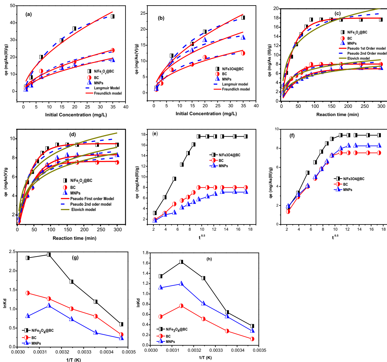
Fig. 4 The equilibrium and kinetic adsorption data modeling (a, b) As(III & V) data modeling via Langmuir and Freundlich model (c,d) As(III & V) data interpretation via Pseudo 1st, 2nd and Elovich model (e, f) As(III & V) data interpretation via Intraparticle model.
