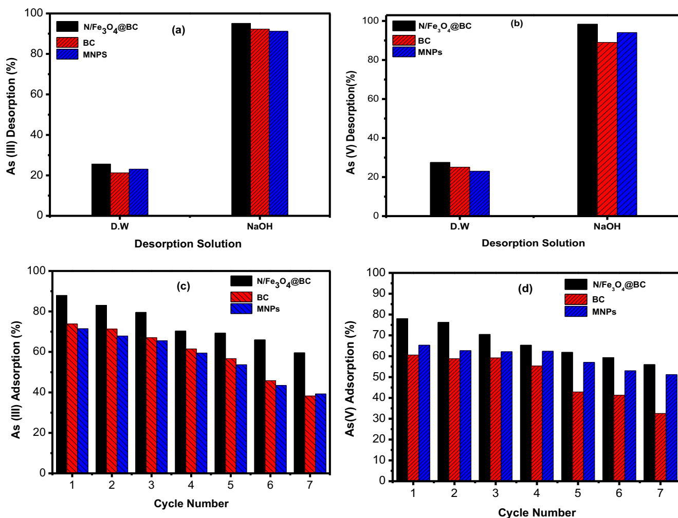
Fig. 5 Desorption performance of all tested adsorbents for As(III) and As(V) (a,b) as well as subsequent adsorption/desorption cycles (c, d) by using distilled water, alkaline eluents.
