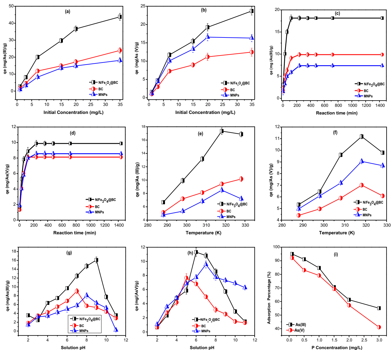
Fig. 3 Adsorption of Arsenic As (III & V) as a function of (a, b) initial concentration (c, d) reaction time (e, f) Temperature (g, h) Solution pH (i) Phosphate concentration.
