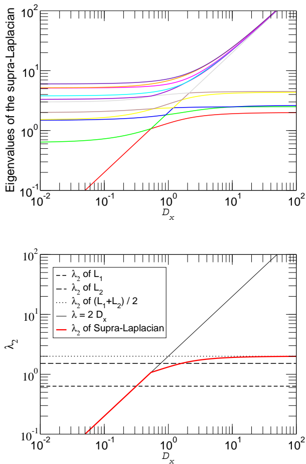
FIG. 2: (color online) Evolution of the eigenspectra of the toy model presented in Fig. 1 as a function of the coupling D_x (top) for D_1 = D_2 = 1 , and comparison between the second smallest eigenvalues \lambda_2 of the different Laplacians (bottom).
