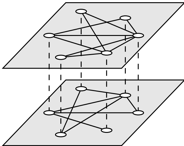
FIG. 1: Example of multiplex network with M = 2 layers. Nodes are the same in both layers. The connectivity at each layer is independent of each other, the connectivity inter-layer is from each node to itself (dashed links).
