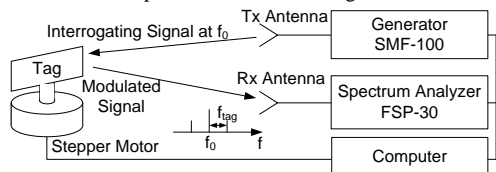
Fig. 11. Experimental setup used to measure the transponder angular response.
