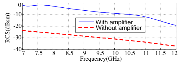
Fig. 7. Simulated RCS of the active transponder as a function of frequency with (solid line) and without (dotted line) the amplifier.
