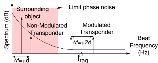
Fig. 2. Baseband spectrum using non-modulated and modulated transponders, in the presence of a parasitic reflector in the vicinity of the transponder.
