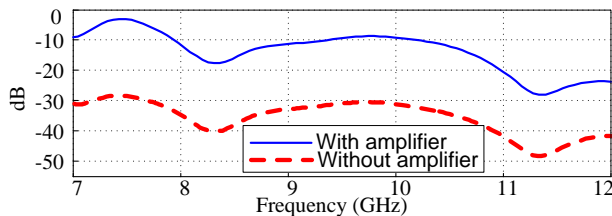
Fig. 6. Simulated open-loop gain without amplifier (dotted line) and with amplifier (solid line).
