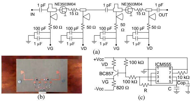
Fig. 4. (a) Circuit schematic of the two-stage amplifier, (b) photograph of the transponder (top view) and the ground reflector and (c) circuit schematic of the oscillator.
