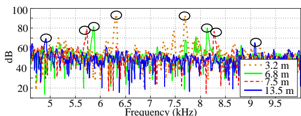
Fig. 9. Measurement of the modulated transponder with f_{tag}=7 kHz using the background subtraction technique.
