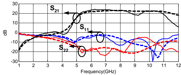
Fig. 5. Measurements (solid line) and simulations (dotted line) of S_{11} , S_{22} and S_{21} parameters of the two-stage amplifier.
