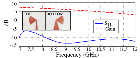
Fig. 3. Simulated reflection coefficient ( S_{11} ) and antenna gain.
