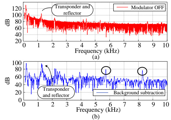
Fig. 8. Measurement of the transponder and dihedral reflector at 8 m (a) in case of no modulation or (b) with f_{tag}=7 kHz modulation.
