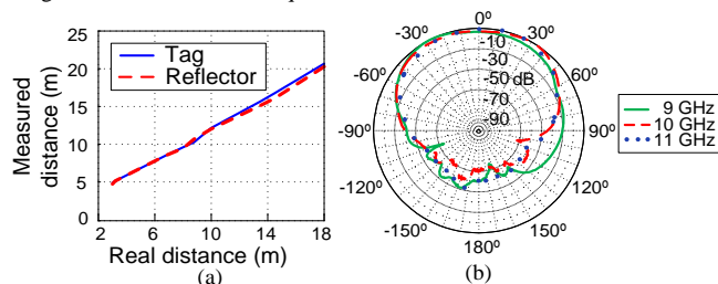
Fig. 10. (a) Measured distance obtained from the dihedral reflector (dashed line) and derived from the spacing between the sideband peaks (solid line). (b) Normalized measured power as function of angle at 9, 10 and 11 GHz.
