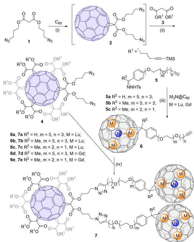
Scheme 1. Synthesis of the MBT Platform 7 . Reagents and conditions: (i) C_{60} , CBr_4 , DBU, toluene, r. t.; (ii) CBr_4 , DBU, toluene, r. t.; (iii) NaOMe, Pyridine, o -DCB, r. t. to 70 °C (for 6a–c ) or 55 °C (for 6d–e ); (iv) CuBr-SMe 2 , sodium ascorbate, Cu 0 , o -DCB, r. t. (for 7a ) or 40 °C (for 7b–e ).
