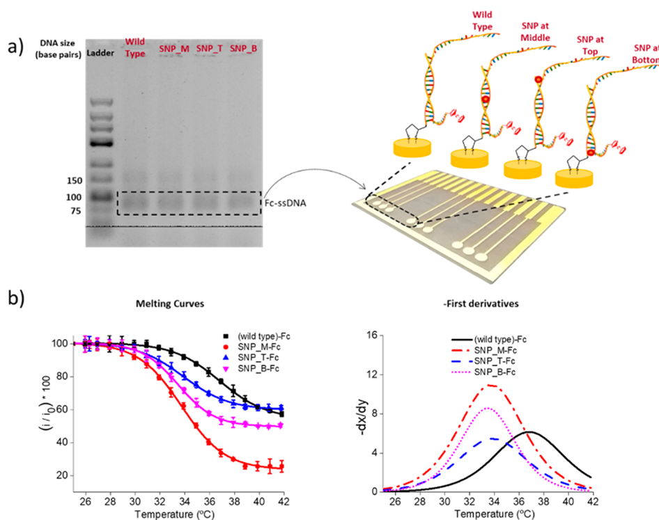
Figure 6. (a) Agarose gel electrophoresis analysis of each of the ssDNA 124-mer amplicons obtained after asymmetric PCR amplification, with the amplicons designed to be fully complementary (wild-type) or to contain a single mismatch designed to be at the top, bottom, or middle of the hybridized duplex. (b) Melting curves obtained for the four different asymmetric PCR targets and the corresponding first derivatives. All measurements were carried out in triplicate.
