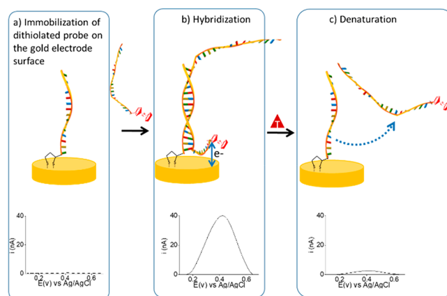
Figure 1. Conceptual schematic representation of the electrochemical melting curve analysis approach: (a) Immobilization of dithiolated probe on the gold electrode surface. (b) Hybridization with single-stranded DNA PCR amplicon containing the SNP to be interrogated. (c) Temperature ramping and denaturation of the surface-tethered duplex and concomitant decrease in the electrochemical signal.
