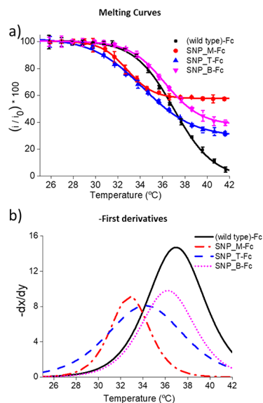
Figure 4. (a) Melting curves and (b) the corresponding first derivatives obtained for four different 21-mer synthetic targets hybridized to a common surface tethered capture probe, with each of the targets being the fully complementary wild-type ((wild type)-Fc) or containing a single mismatch at middle (SNP_M-Fc), top (SNP_T-Fc), or bottom (SNP_B-Fc) of the sequence. All measurements were carried out in triplicate.
