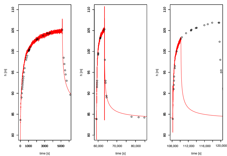
Figure 12. Validation. 2nd set of parameters. Water level evolution. Zoom.
