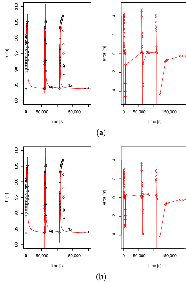
Figure 11. Validation. (a) Left, water level evolution, measured (black) and simulated (red) with the 1st set of parameters (updated). Right, error estimation evolution. (b) Same results as (a) with the 2nd set of parameters (updated).
