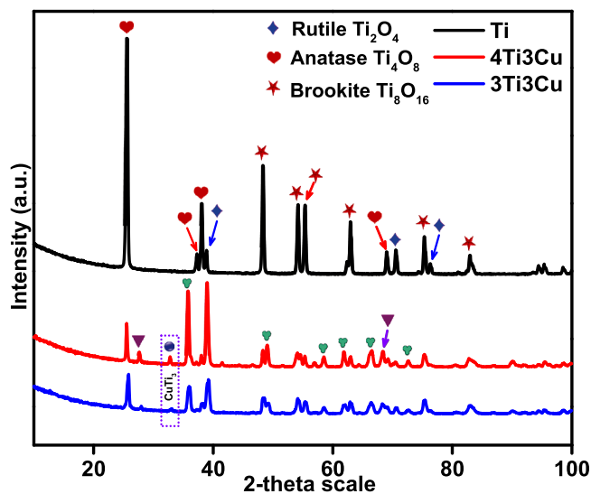
Fig. 3. XRD pattern for the Ti-Cu nano-catalysts.
