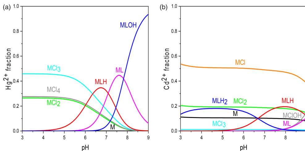
Fig. 2 Speciation diagrams vs. pH of (a) Hg 2+ - and (b) Cd 2+ -CAR (L) species (charges omitted for simplicity) in NaCl aqueous solution at I = 0.15 mol L -1 and T = 298.15 K (C M = 2 mmol L -1 ; C L = 4 mmol L -1 ).
