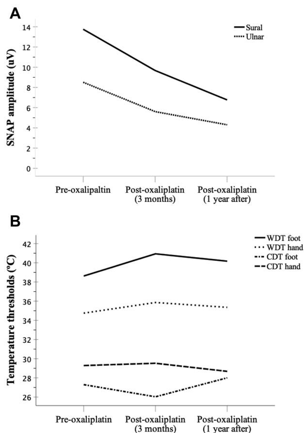
Fig. 4 Time profile reflecting the change in NCS and TST from baseline to one-year follow-up. The line chart shows mean values of SNAP amplitude ( A ) and temperature ( B ) for warm and cold thresholds at foot and hand corresponding to the patients who were followed one year after last oxaliplatin cycle of chemotherapy. Amplitudes are expressed in microvolts and temperature in Celsius degrees
