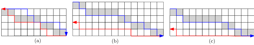
FIGURE 9 Figures (a)– (c) show the matrices A_{5,11} , A_{6,15} , and A_{5,14} , respectively, with chessboards (2, t + 3, 2, 2) for t = 1 (a), (2, t + 3, 2, 3, 2) for t = 2 (b), and (2, t + 3, 2, 3) for t = 3 (c). We observe that for the pair of Top and Bottom travels described in these matrices, A_{5,11} has only one interior element (column 1), A_{6,15} has only two interior elements (columns 13 and 15), and A_{5,14} has only three interior elements (columns 11,13, and 14).
