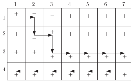
FIGURE 2 Top and Bottom travels in matrix A.
