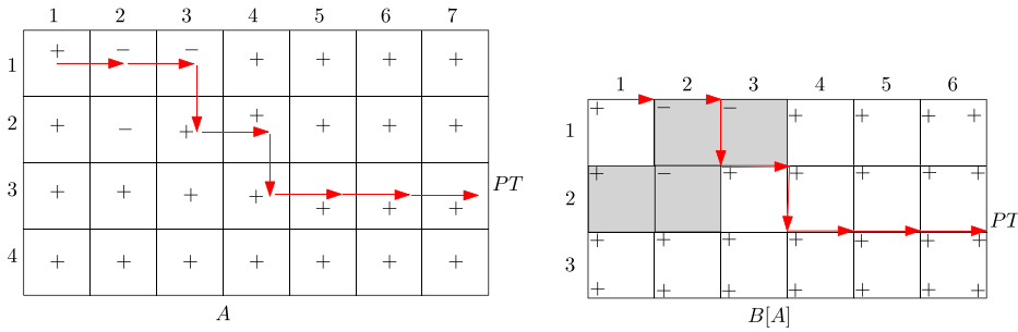
FIGURE 3 A matrix A and its chessboard B[A] with the same plain travel PT .
