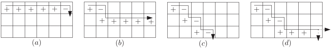
FIGURE 1 The TT of (a)–(d) satisfies the situations 2(a)–2(d), respectively, of the definition of the Top Travel.
