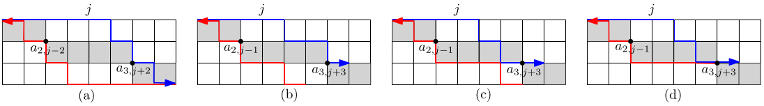
FIGURE 5 The chessboard with sequence (2, t + 3, 2) considered in Theorem 4.4, for t = 1 . Figure (a) shows the case when BT arrives at the j th column at row 4, for j = 5 , and figures (b)–(d) consider the cases when BT arrives at the j th column at row 3, for j = 4 .
