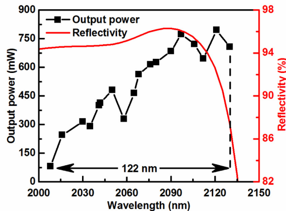
Fig. 3. Spectral tunability of the CW Ho:YAG ceramic laser obtained with a Lyot filter (1.5% OC) and reflectivity curve of the used GaSb-based SESAM.
