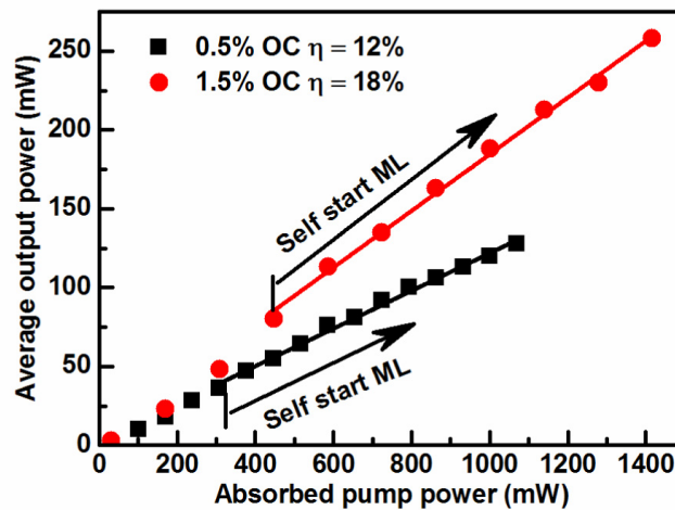
Fig. 4. Output power versus absorbed pump power of the mode-locked Ho:YAG ceramic laser for different output couplers (OCs) without the Lyot filter in the cavity. The vertical lines indicate the transition from CW to clean mode-locked operation (ML – mode locking).
