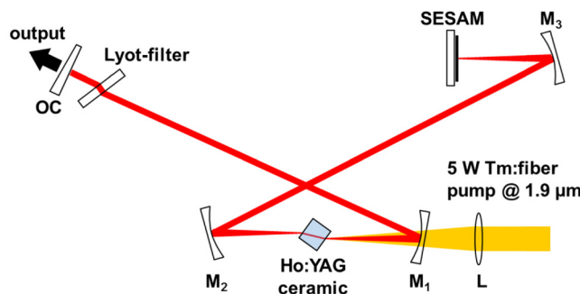
Fig. 2. Scheme of the mode-locked Ho:YAG ceramic laser (L: lens; M1-M3: dichroic folding mirrors; OC: output coupler; Lyot-filter: birefringent filter).
