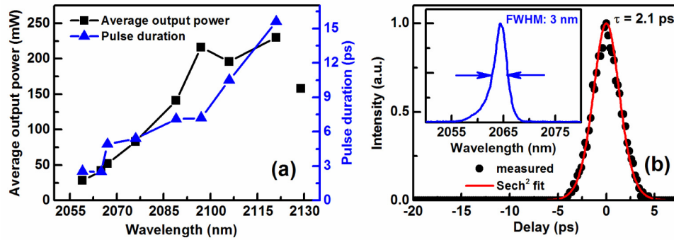
Fig. 6. (a) Spectral tunability of the mode-locked Ho:YAG ceramic laser with the Lyot filter in the cavity (1.5% OC), (b) Autocorrelation trace and emission spectrum (inset) of the shortest pulses (0.5% OC).
