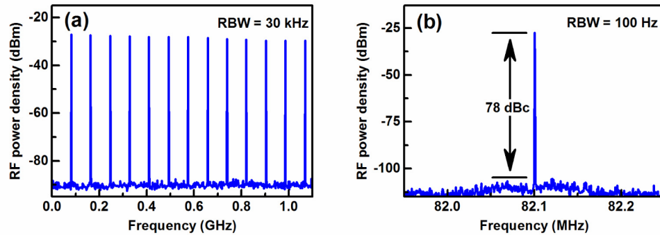
Fig. 7. Radio frequency spectra of the SESAM mode-locked Ho:YAG ceramic laser: (a) 1.1 GHz wide-span, (b) fundamental beat note (RBW: resolution bandwidth).
