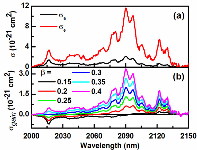
Fig. 1. Spectroscopic characterization of the 1% Ho-doped YAG ceramics in the 2- \mu\text{m} region. (a) Absorption \sigma_a and emission \sigma_e cross section. (b) Gain cross section \sigma_{\text{gain}} for different inversion levels \beta .
