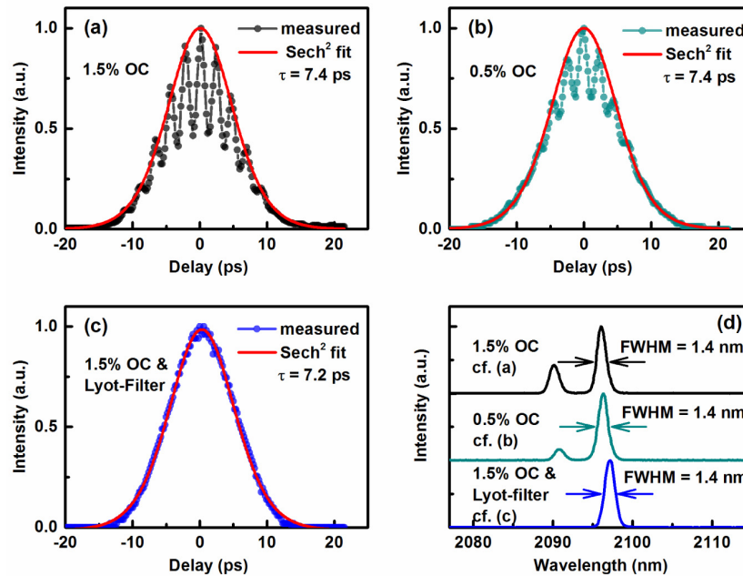
Fig. 5. SESAM mode-locked Ho:YAG ceramic laser. Autocorrelation traces without (a,b) and with a Lyot filter (c) in the cavity (OC: output coupler). (d) Emission spectra corresponding to (a), (b) and (c).
