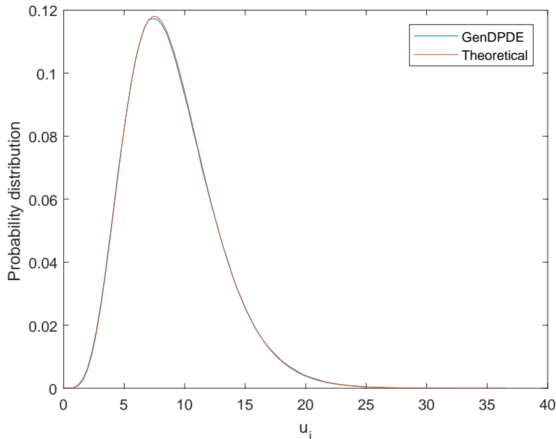
FIG. 2: Equilibrium particle internal energy probability distribution from a GenDPDE simulation of mesoparticles fixed in space using a small constant-volume heat capacity C_V = 5k_B , with initial system temperature T = 1.5 , system particle density \rho = 0.5 , and heat conductivity parameter \kappa = 1 . The theoretical distribution was determined from eq. (65).
