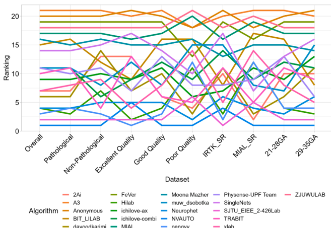
Fig. 7. Ranking of each algorithm for each subset of data in Section 3.3.
