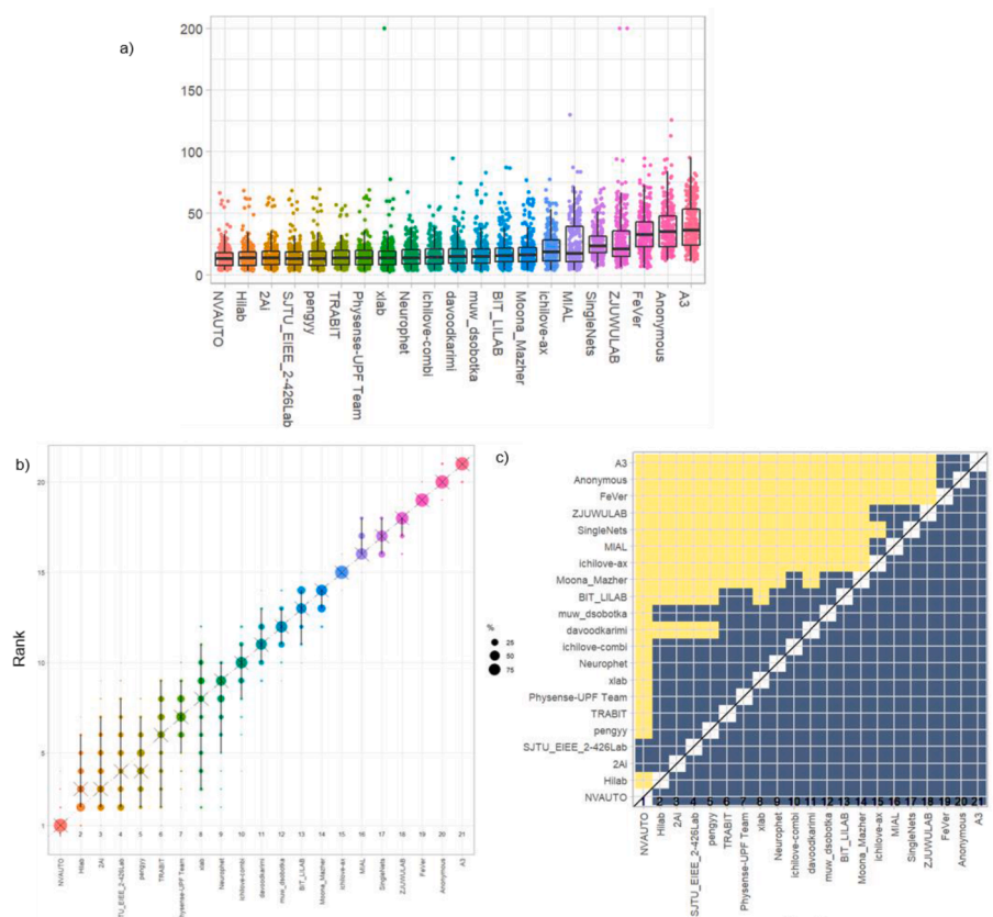
Fig. 5. HD95 values of FeTA Challenge participants a) Dot and box plot; b) Blob plot for visualizing ranking stability based on bootstrap sampling, black cross indicated the median rank for each algorithm and 95% bootstrap intervals across samples are indicated by black lines; c) Significance maps for visualizing ranking stability based on statistical significance (Yellow: metrics from the algorithm on the x-axis were significantly superior to the algorithm on the y-axis, blue color indicates no significant difference.).
