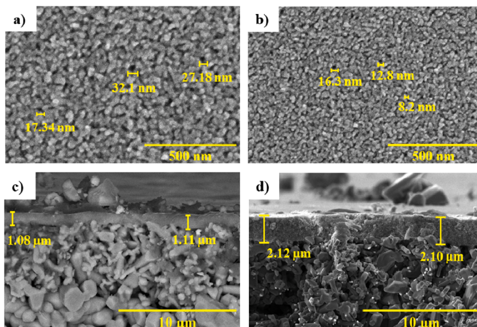
Fig. 5. FESEM microscopy images a-b) the surface of TCSCM and TCSGOM, and c-d) the cross-section of TCSCM and TCSGOM (TCSCM: 10 % wt. Matrimid and TCSGOM: 1 mg·L -1 GO solution).
