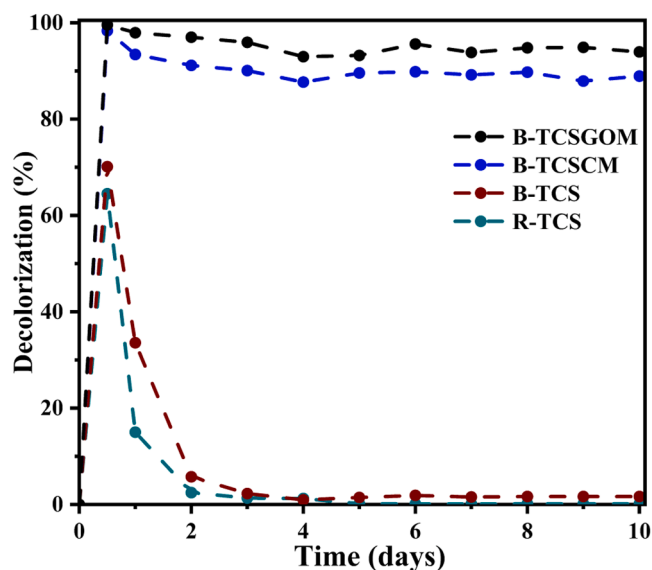
Fig. 7. Anaerobic decolorization of AO7 in TCS reactor and TCS, TCSCM, and TCSGOM bioreactors. Flux = 0.10 \text{ L} \cdot \text{m}^{-2} \cdot \text{h}^{-1} , [\text{AO7}]_0 = 50 \text{ mg} \cdot \text{L}^{-1} and T = 37^\circ \text{C} .
