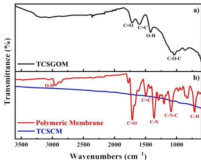
Fig. 3. FTIR analysis of the a) TCSGOM and b) polymeric precursor membrane and TCSCM (TCSCM: 10 % wt. Matrimid and TCSGOM: 1 \text{ mg}\cdot\text{L}^{-1} GO solution).
