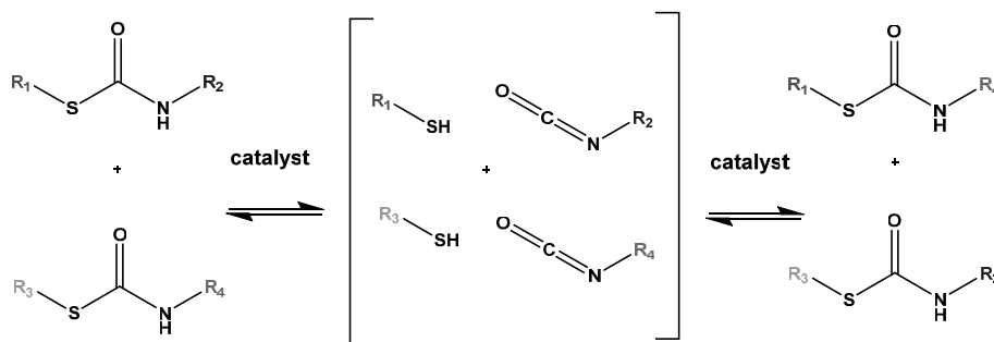
Scheme 3. Proposed mechanism of trans -thiocarbamoylation exchange process.
