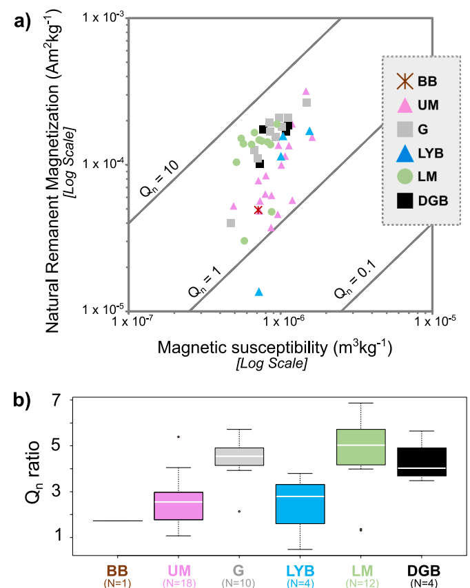
Fig. 2. Koenigsberger ( Q n ) values by facies. (a) Intensity of the natural remanent magnetization (NRM) vs. magnetic susceptibility on a mass-specific basis. Isolines indicate constant Q n values from 0.1 to 10. Facies are denoted according to the legend. (b) Box-plot distinguishing the Q n values by facies indicating the number of specimens analysed.
