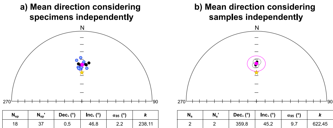
Fig. 7. Equal area projections showing the mean direction (pink circle) calculated at (a) specimen and (b) sample level, respectively. The 95% circle of confidence or \alpha_{95} is shown in pink. Yellow star indicates the expected field direction. In panel a, specimens from block 1 and 2 are shown in black and blue, respectively. [ N_{sp}/N_s = number of specimens/samples considered to calculate the mean direction; N_{sp}'/N_s' = number of specimens/samples analysed; Dec. = declination; Inc. = inclination; \alpha_{95} = 95 per-cent confidence cone of mean direction and k , precision parameter according to Fisher (1953)].
