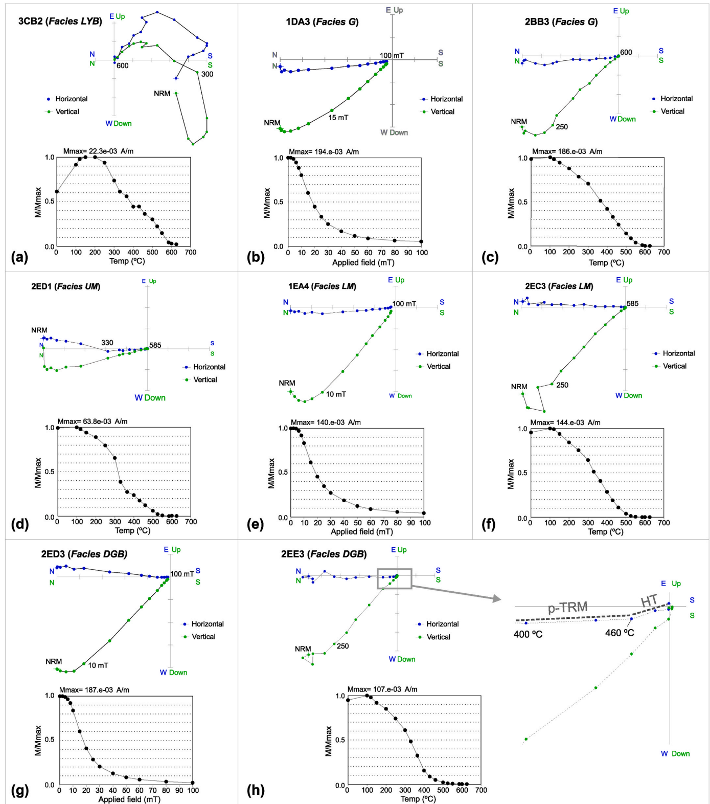
Fig. 6. (A–h). Orthogonal NRM demagnetization plots of representative specimens from different facies. Blue (green) circles show projections of vector endpoints onto the horizontal (vertical) plane. The specimen code, facies, intensity (NRM 0 ) and normalized intensity decay curves are shown for each specimen. In Fig. 6h, the final steps of the diagram are blown up to show the presence of a high-temperature (HT) component. p-TRM = partial thermoremanence.
