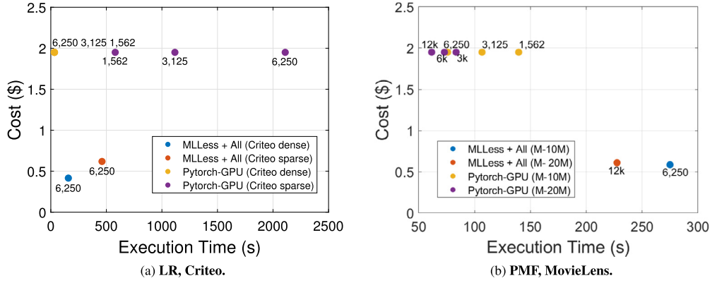
Fig. 11. Cost-performance comparison between PyTorch running on a GPU (PyTorch-GPU) and MLLess with all optimizations (MLLess+All).
