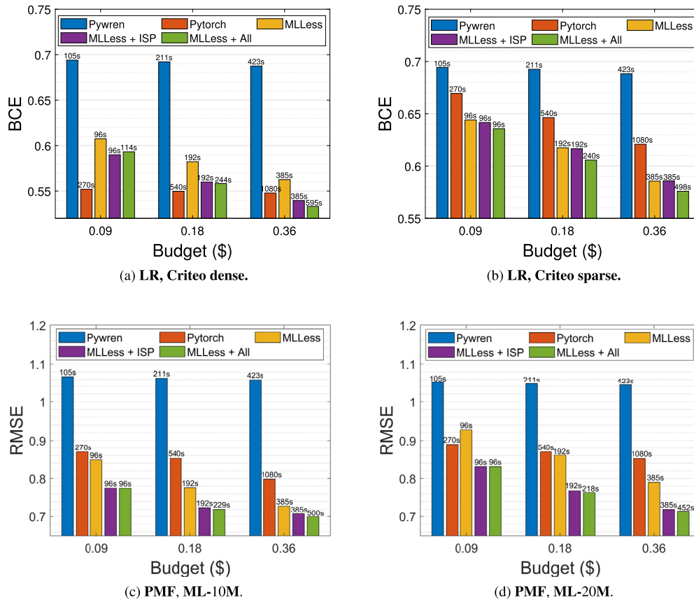
Fig. 10. Cost vs. loss comparison between PyTorch, PyWren-IBM and MLLess with different variants: BSP synchronization ( MLLess ), ISP synchronization ( MLLess + ISP ) and ISP synchronization + auto-tuner ( MLLess + All ), for 24 workers. The numbers above the bars report the maximum execution time affordable with each possible budget.
