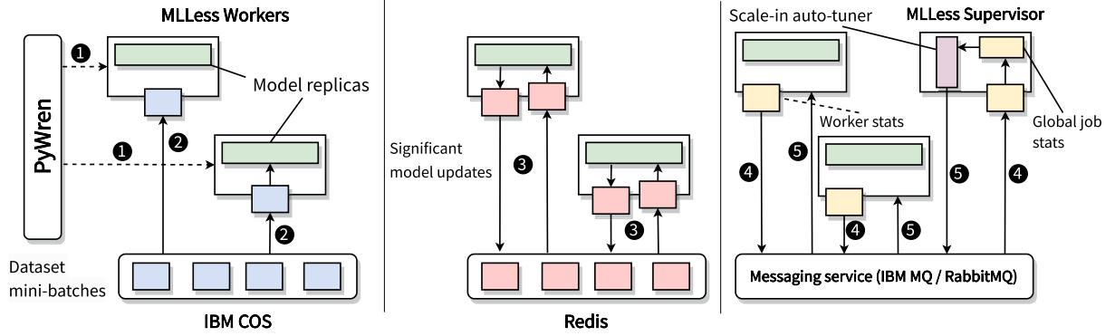
Fig. 2. Typical execution of a training job with MLESS.
