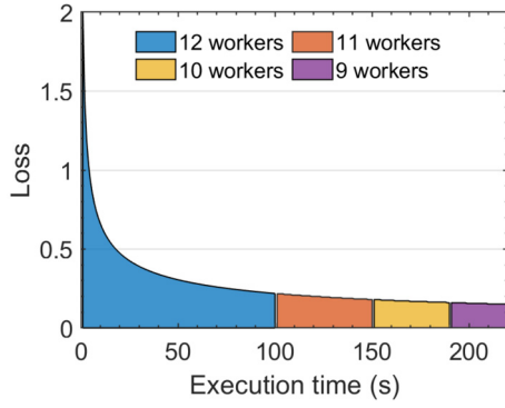
Fig. 3. Sample execution of the scale-in scheduler. In the low convergence zone, workers are progressively removed from the pool.
