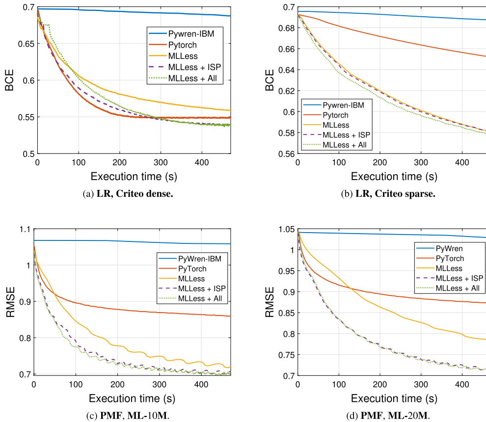
Fig. 9. Loss vs. time comparison between PyTorch, PyWren-IBM and MLLess with different variants: BSP synchronization (MLLESS), ISP synchronization (MLLESS + ISP) and ISP synchronization + auto-tuner (MLLESS + All), for 24 workers.
