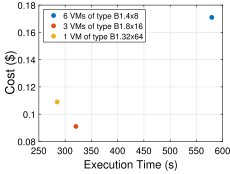
Fig. 6. Cost-performance comparison of PyTorch using different IaaS setups for PMF on MovieLens-10M dataset.
