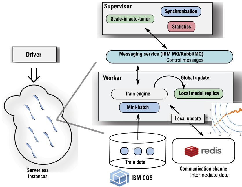
Fig. 1. MLLess system architecture.
