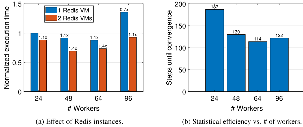
Fig. 13. Scalability of MLLess on the ML-20M dataset.
