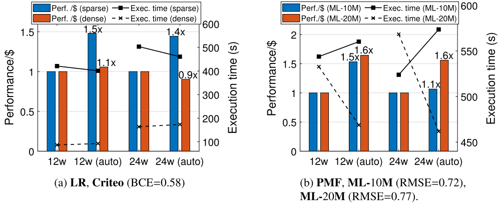
Fig. 8. Effect of the scale-in auto-tuner. Two metrics are used: Perf/$ (bars; left axis); execution time (lines; right axis).
