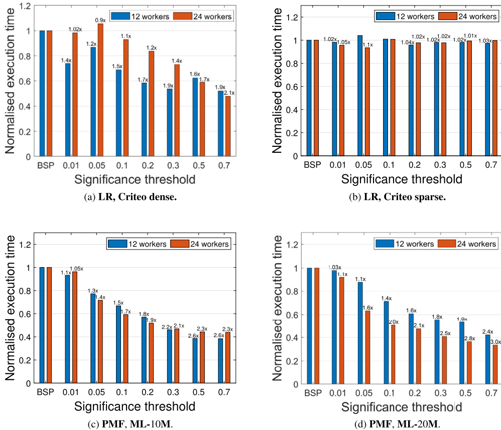
Fig. 7. Normalized execution time until convergence as the significance threshold \nu increases.
