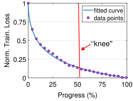
(b) Reference curve fitting: \theta_0 = 0.05 , \theta_1 = 1.58 , \theta_2 = 0.58 , \theta_3 = 0.49 .
