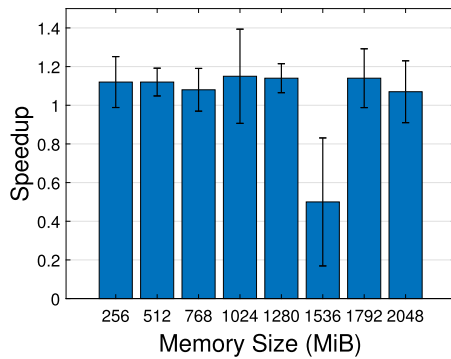
Fig. 5. Speedup of two threads relative to single-thread performance within a function as memory size is varied.
