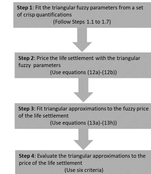
Fig. 2. Steps of the fuzzy framework to price LSs. Source: Own elaboration.
