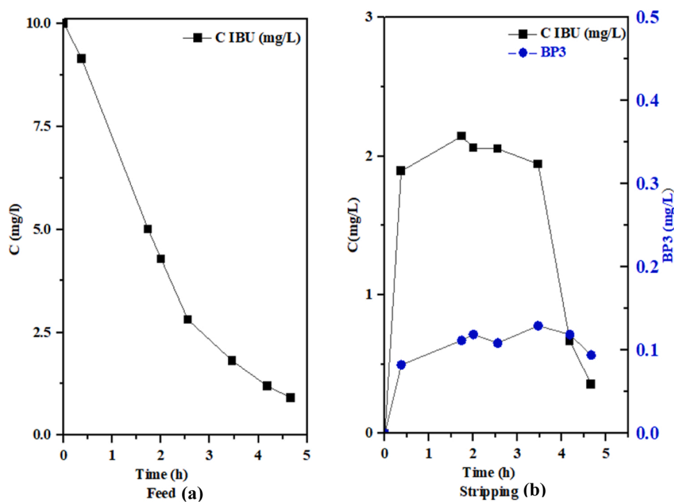
Fig. 13. Concentration of IBU and by-product BP3 in (a) Feed: C_0 = 10 mg/L, V = 9 L, Q = 47 L/h, pH = 5.5; Organic extractant: 40% (v/v) Cy923/kerosene (b). Stripping phase: V = 2 L; pH = 11; Q = 47 L/h; Inlet ozone concentration 10.2 mg O_3 /L.
