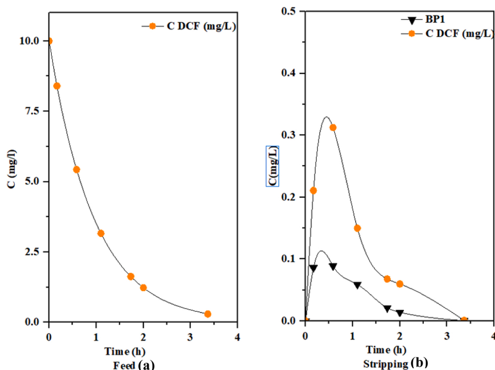
Fig. 12. Concentration of DCF and by-product BP1 in (a) Feed: C_0 = 10 mg/L, V = 9 L, Q = 47 L/h, pH = 5.5; Organic extractant: 40% (v/v) Cy923/kerosene (b). Stripping phase: V = 2 L; pH = 11; Q = 47 L/h; Inlet ozone concentration 10.2 mg O_3 /L.
