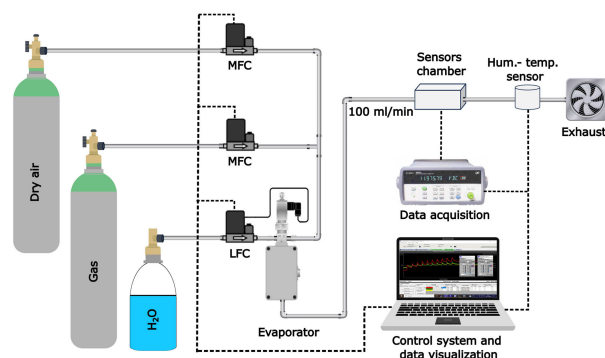
Fig. 2. Schematic illustration of gas measurement system used to evaluate the gas detection performance of manufactured sensors.
