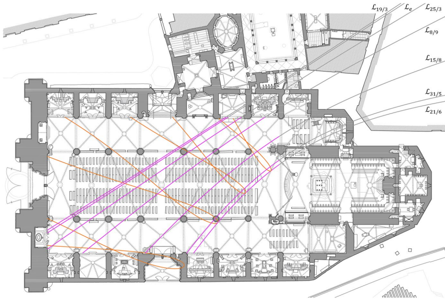
Fig. 9 Graphical representation of \mathcal{L}_{19/3} , \mathcal{L}_e , \mathcal{L}_{25/3} , \mathcal{L}_{8/9} , \mathcal{L}_{15/8} , \mathcal{L}_{31/5} and \mathcal{L}_{21/6} on the cathedral's floor plane \rho
