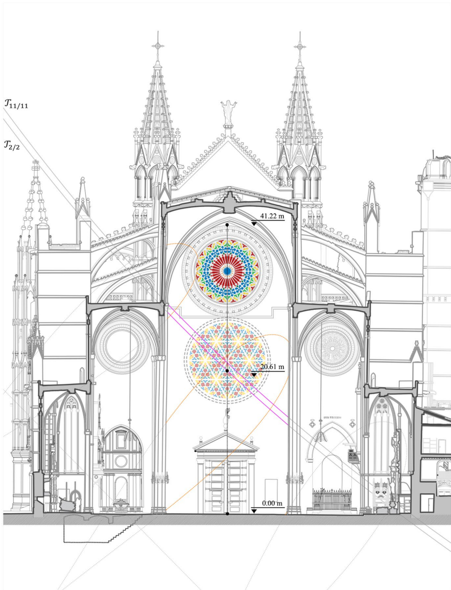
Fig. 6 Graphical representation of T_{11/11} and T_{2/2} on the plane \sigma
