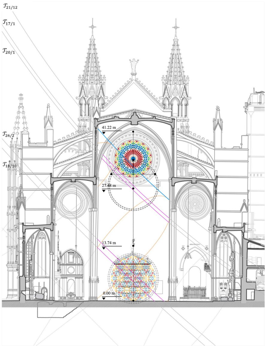
Fig. 8 Graphical representation of T_{21/12} , T_{17/1} , T_{20/1} , T_{26/2} and T_{18/10} on the plane \sigma
