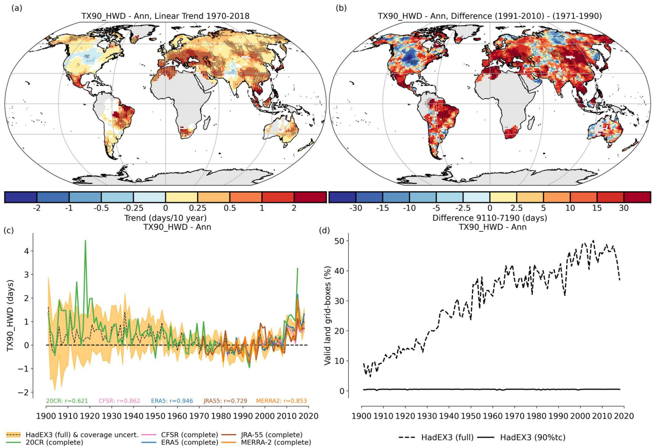
Figure 4. Maps of trends and differences, and time series of the global average and coverage for TX90-HWD (heat wave duration, days), using 1981–2010 as the reference period for the calculation of the 90th percentile. Regions shown in white in (a) have values of zero throughout the record. No time series is calculated using temporally complete grid boxes for this index. No 90% temporal complete version of HadEX3 is shown in (c) because periods where this index is undefined (i.e., no heat waves occurred) mean this criterion is met much less often than for other indices, as shown in panel (d) (see Section 4.1).
