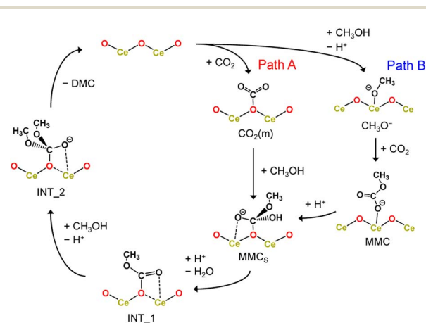
Fig. 4 Reaction mechanism of DMC formation from CO 2 and methanol. Path A starts with an adsorbed CO 2 molecule while Path B starts from the dissociative adsorption of a methanol molecule.
