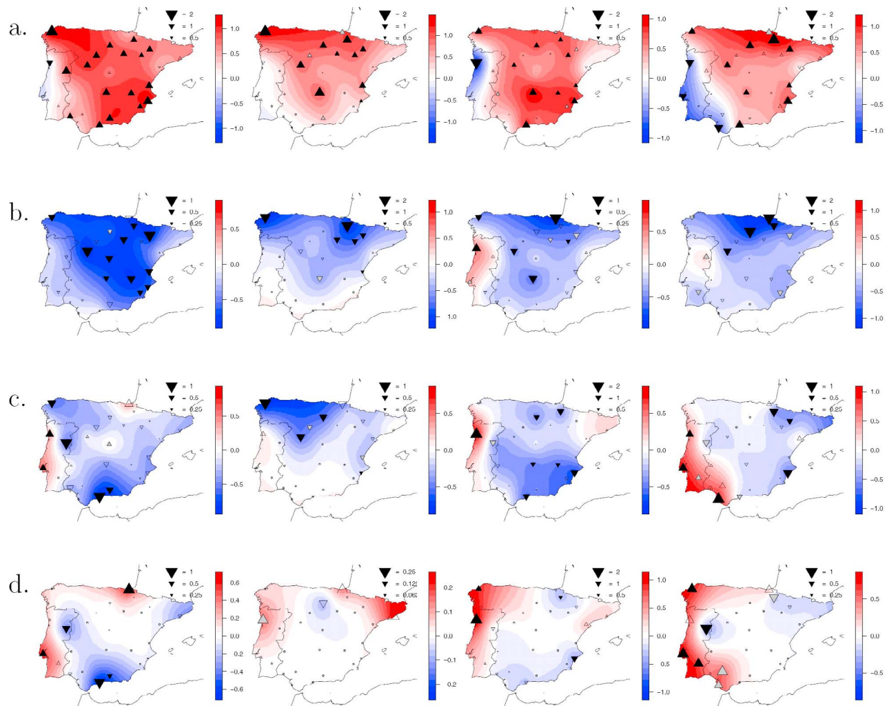
Figure 10. Mann-Kendall test for proportion of rainy days in each rainfall category with respect to the total in (from left to right) spring, summer, fall, and winter: (a) light, (b) moderate, (c) intense, and (d) very intense. Upward-pointing triangles represent increasing trends, and downward-pointing triangles represent decreasing trends. The size of each triangle is proportional to the magnitude of the normalized trend (normalized by the standard deviation). Solid black triangles represent trends significant at the 5% level, and solid gray triangles indicate trends significant at the 10% level. Isolines correspond to interpolated values of the normalized trend (in percentage). Circles show trends with absolute value of <0.125 . Period is 1903–2003.
