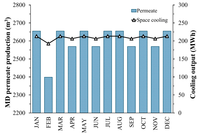
Fig. 13. Monthly permeate production and cooling output-for-space cooling applications of the proposed ST-AHP-MD system with auxiliary heater.
