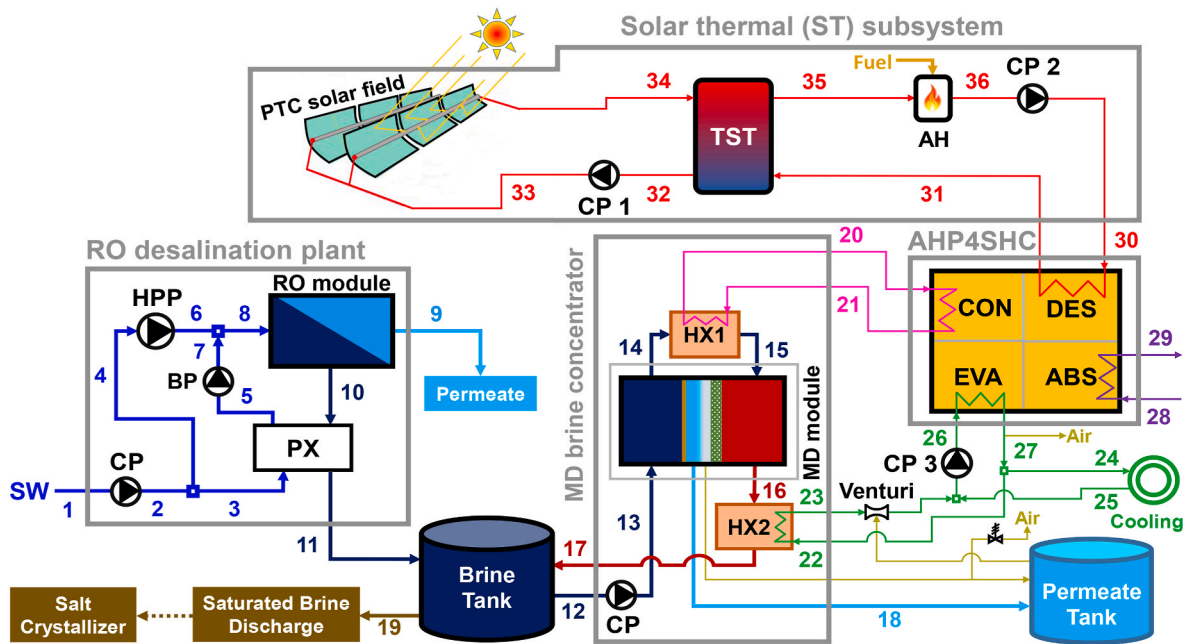
Fig. 1. Solar-powered AHP integrated with MD desalination system with feed brine recirculation for sustainable RO desalination brine concentration and space cooling applications.
