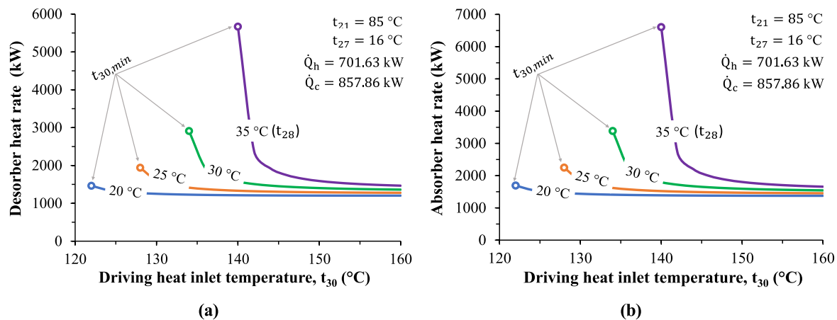
Fig. 8. Effect of driving heat temperature ( t_{30} ) at several absorber cooling water temperatures ( t_{28} ) on (a) desorber heat rate and (b) absorber heat rate of the AHP for simultaneous heating and cooling supplies.
