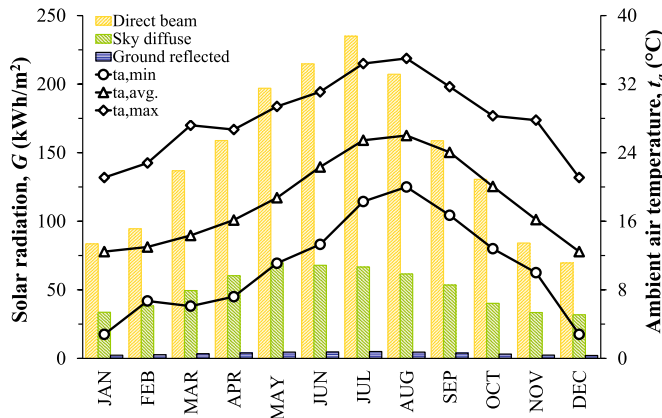
Fig. 10. Monthly variation of solar radiation and ambient air temperature of Almería (Spain) [48].
