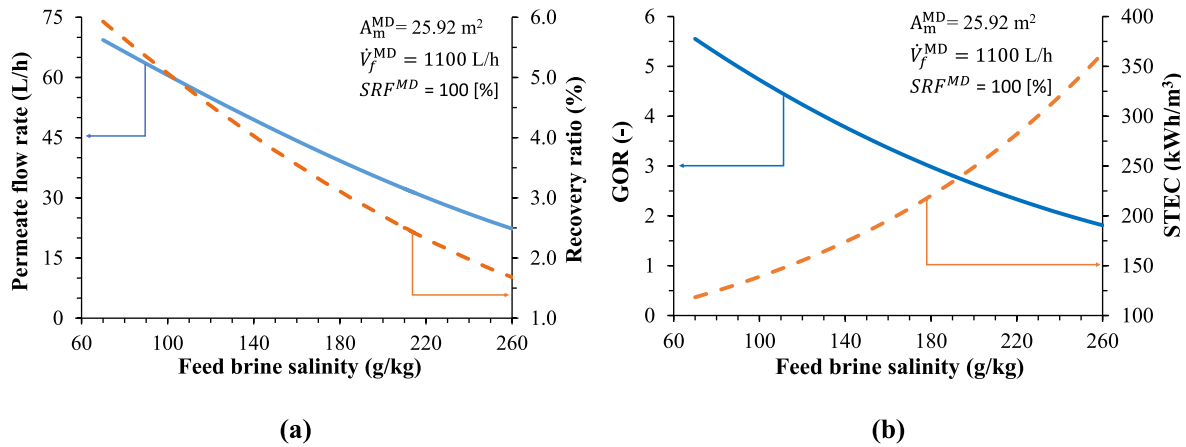
Fig. 5. Effect of feed brine salinity for a single-pass MD system based on Aquastill AS26 AGMD module on (a) permeate production rate and recovery ratio and (b) GOR and STEC.
