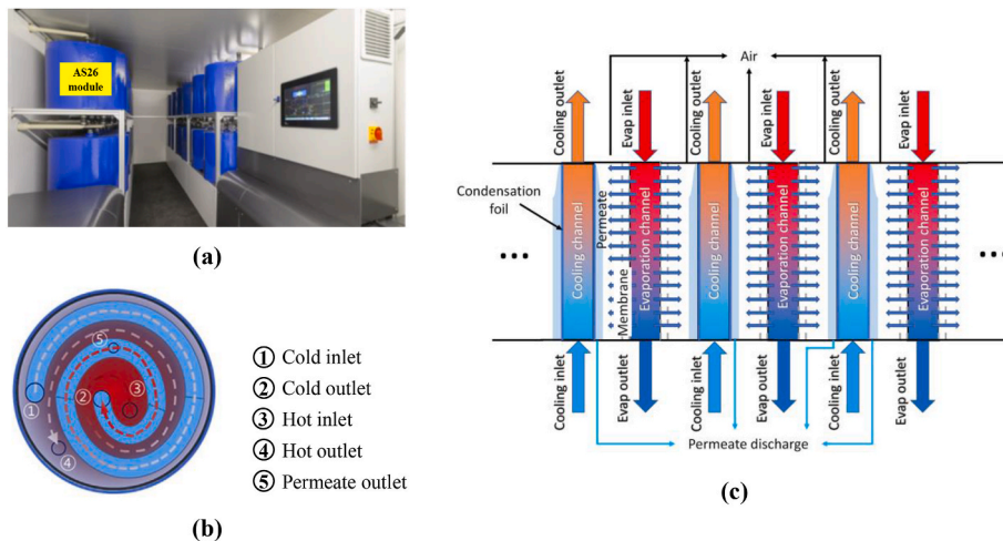
Fig. 2. (a) Aquastill PURA-100 system using AS26 AGMD module, adapted from Ref. [29], (b) cross sectional view of Aquastill AGMD module adapted from Ref. [30], and (c) internal arrangement of a multi-envelope spiral-wound V-AGMD module, adapted from Ref. [31].
