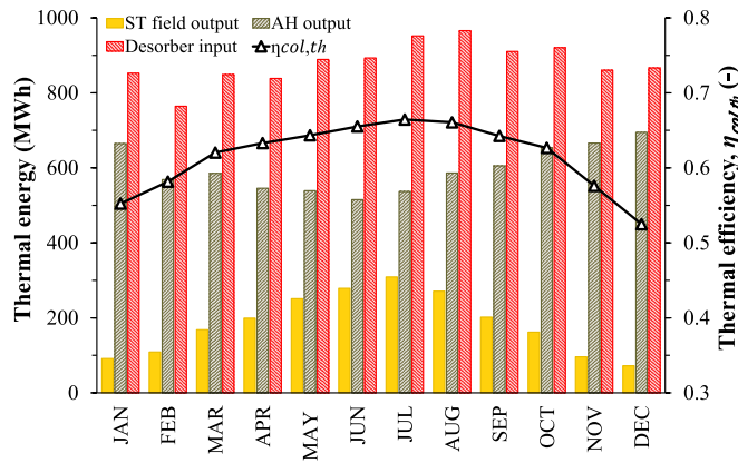
Fig. 11. ST field useful heat output and thermal efficiency, auxiliary heater (AH) output heat, and desorber heat input monthly variation of the ST-AHP-MD system (ST field of 1980 \text{ m}^2 aperture area).
