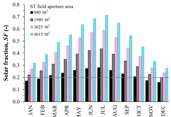
Fig. 9. Effect of solar field area on the solar fraction of the ST-AHP-MD system with auxiliary heater.
