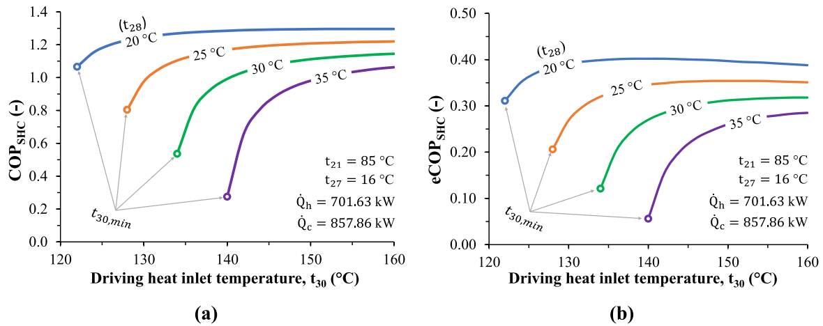
Fig. 7. Effect of AHP driving heat temperature ( t_{30} ) at several absorber cooling water inlet temperatures ( t_{28} ) on (a) COP and (b) eCOP for simultaneous heating and cooling supplies.
