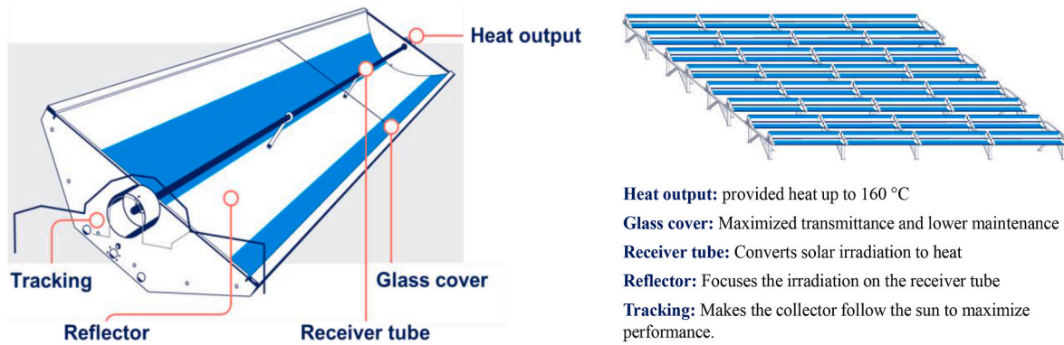
Fig. 4. Absolicon T160 collector with its key component description, adapted from Ref. [34].
