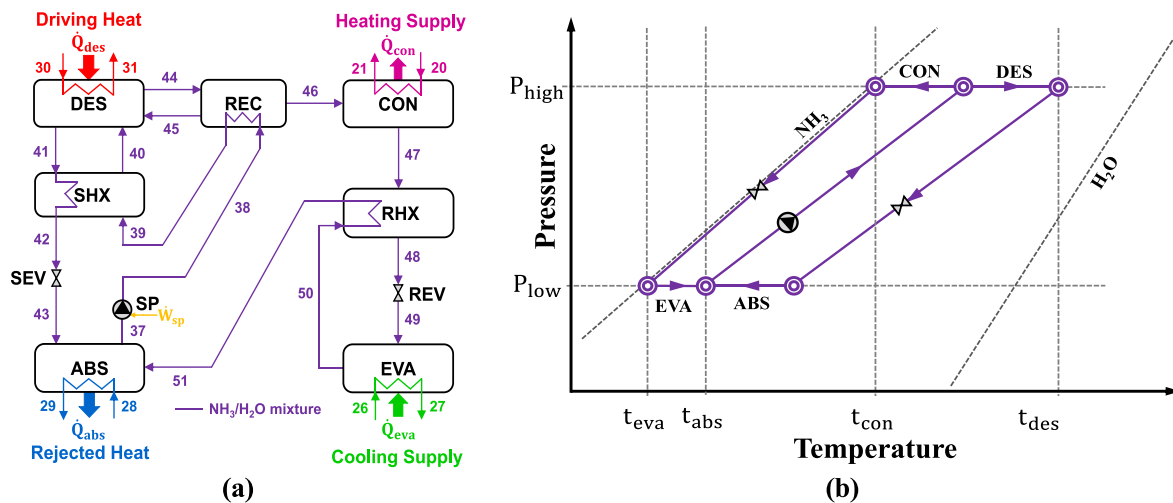
Fig. 3. Single-stage NH 3 /H 2 O AHP for simultaneous heating and cooling applications (a) cycle schematic and (b) cycle representation on pressure-temperature diagram.
