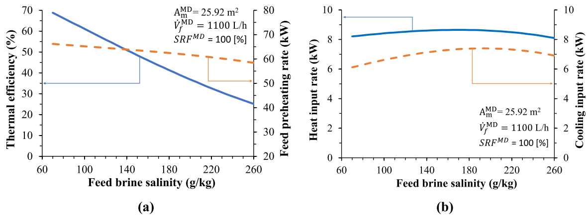
Fig. 6. Effect of feed brine salinity for a single-pass MD system using the Aquastill AS26 AGMD module on (a) thermal efficiency and condenser channels preheating rate and (b) external heat input and cooling input rates.
