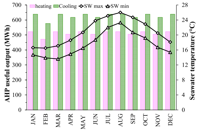
Fig. 12. Monthly absorption heat pump (AHP) simultaneous heating and cooling outputs and seawater temperature range of Almería (Spain).
