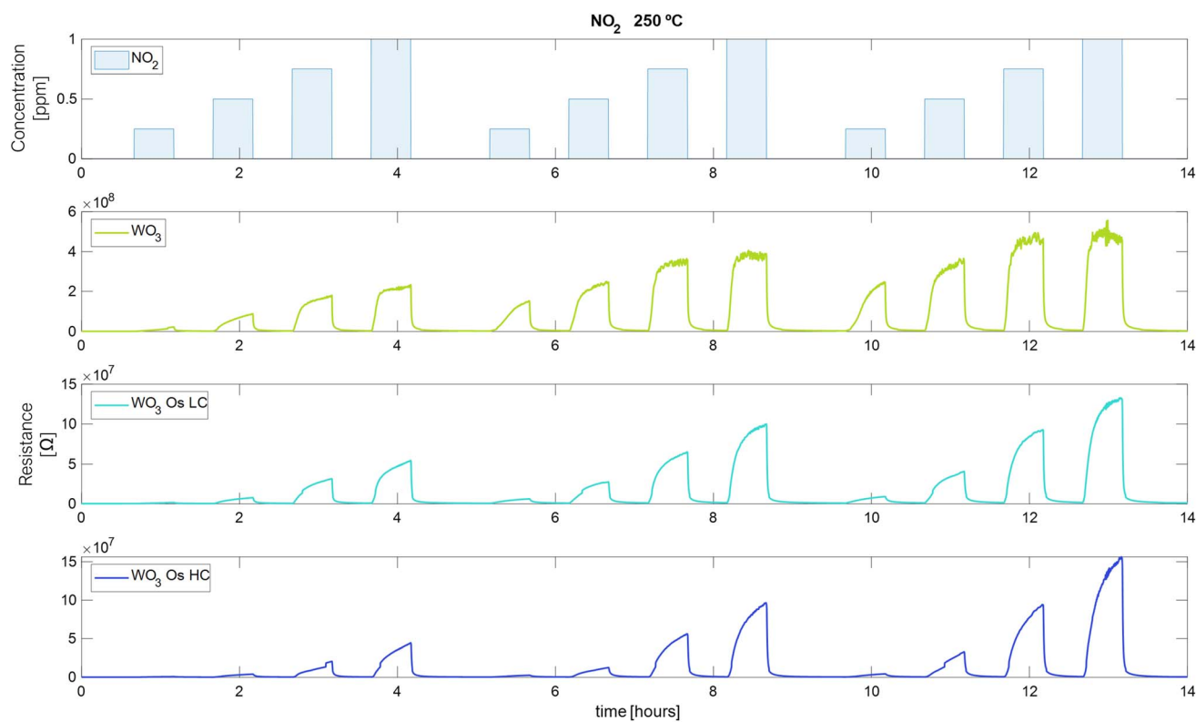
Fig. 8 Measurement of the sensor at an operating temperature of 250 °C throughout \text{NO}_2 exposures.
