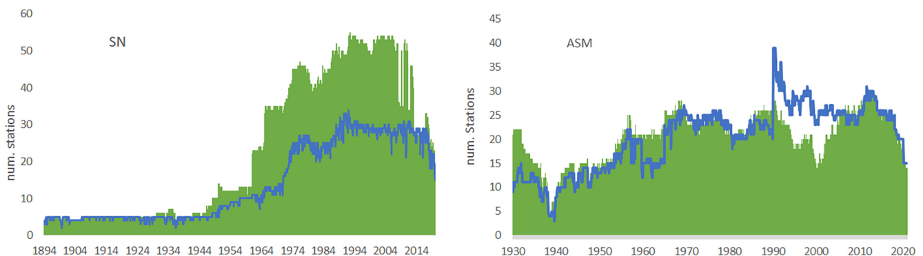
FIGURE 2 Amount of available data for annual temperature and precipitation series in the Sierra Nevada (SN; left) and the Pyrenees (ASM; right). The blue line indicates the availability of stations with temperature series. The green columns indicate the availability of precipitation series.
