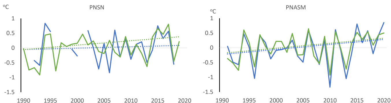
FIGURE 6 Annual average temperature anomalies in highland (blue) and lowland (green) areas in SN (left) and ASM (right) for the 1990–2020 period.
