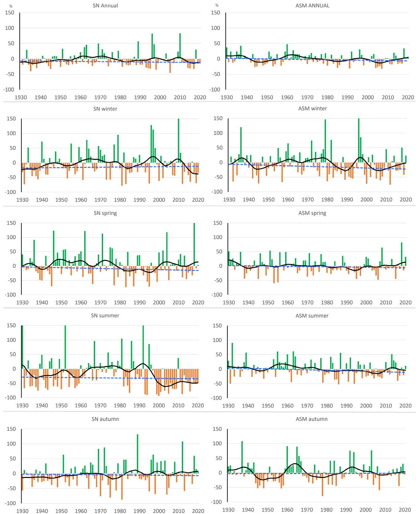
FIGURE 5 Same as Figure 4 but for precipitation. The blue line indicates the trend for the entire period.
