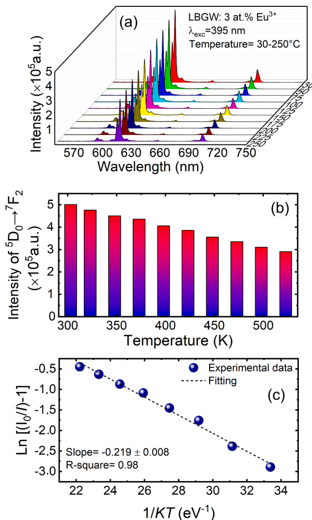
Fig. 12. (a) Emission spectra of the prepared LBGW: 3 at.% \text{Eu}^{3+} phosphors measured at various temperatures; (b) Evolution of the intensity of ^5D_0 \rightarrow ^7F_2 transition as function of the temperature; (c) The relationship of \ln[(I_0/I)-1] versus 1/kT of LBGW: 3 at.% \text{Eu}^{3+} phosphors.
