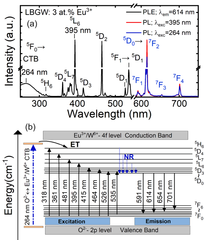
Fig. 7. (a) The photoluminescence excitation (PLE; \lambda_{\text{em}} = 614 nm) and photoluminescence (PL; \lambda_{\text{exc}} = 264 nm and 395 nm) spectra of for LBGW: 3 at.% \text{Eu}^{3+} phosphors. (b) The energy level diagram.
