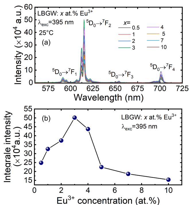
Fig. 8. (a) Emission spectra of LBGW: x at.% \text{Eu}^{3+} ( 0.5 \leq x \leq 10 ) phosphors, \lambda_{\text{exc}} = 395 nm; (b) PL as a function of \text{Eu}^{3+} concentration.
