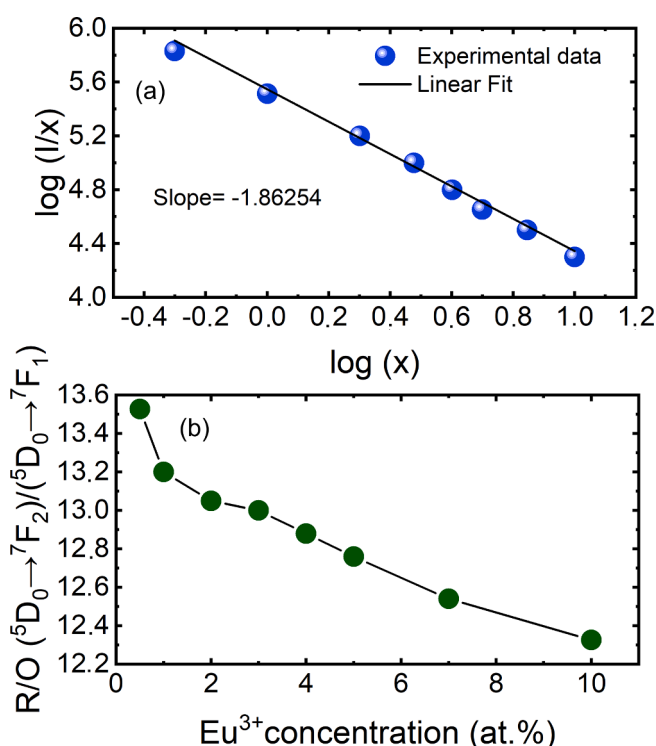
Fig. 9. (a) Dependence of \log(I/x) on \log(x) for of LBGW: x at.% \text{Eu}^{3+} with \lambda_{\text{exc}} = 395 \text{ nm} (b) Asymmetry ratio values with different concentrations levels of \text{Eu}^{3+} ions.
