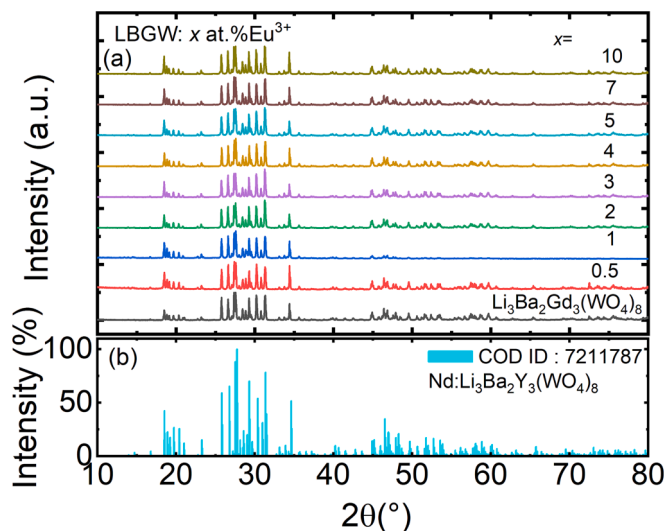
Fig. 1. (a) X-ray diffraction (XRD) patterns of LBGW with different doping concentrations of Eu 3+ ions (0.5–10 %); (b) standard powder diffraction card of Nd: Li 3 Ba 2 Y 3 (WO 4 ) 8 , COD ID:7211787.
