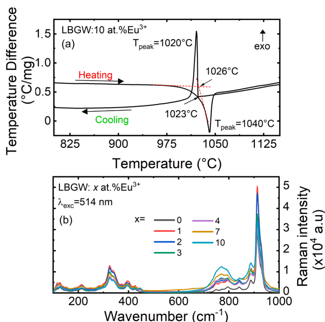
Fig. 4. DTA curves for LBGW: 10 at. \% \text{Eu}^{3+} ; (b) Raman spectra of \text{Li}_3\text{Ba}_2\text{Gd}_3(\text{WO}_4)_8 : x \text{ at.}\% \text{Eu} phosphors, x = 0, 1, 2, 3, 4, 7 and 10 at.%.
