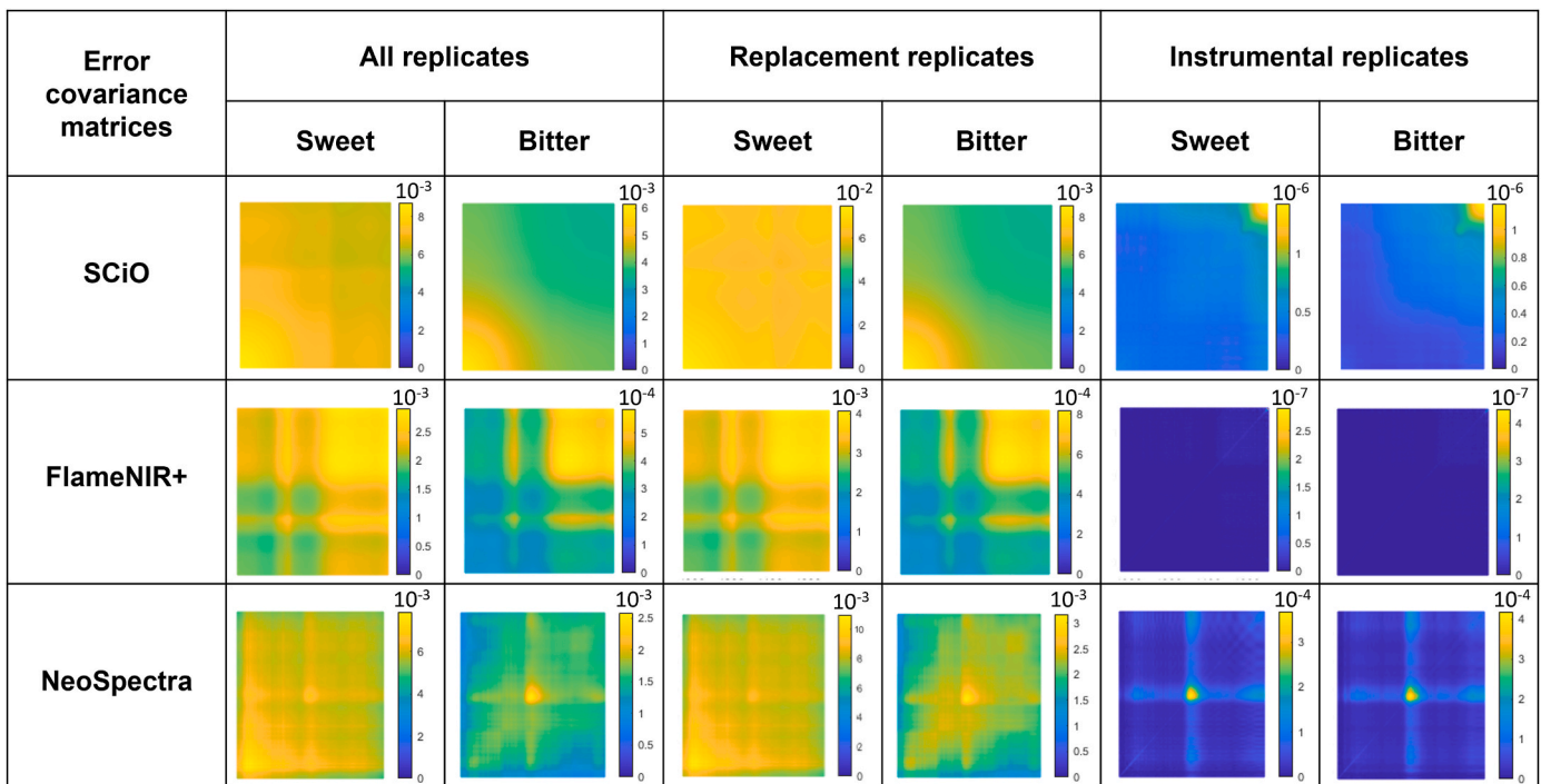
Fig. 3. Error covariance matrices for the SCiO, FlameNIR+ and NeoSpectra spectrophotometers considering different types of replicates: replacement, instrumental and both; averaging the matrices for sweet and bitter almonds separately.
