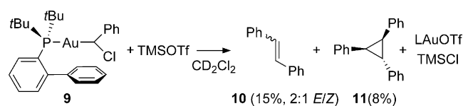
Scheme 4. Activation of complex 9 with TMSOTf. Yields determined by GC-FID.
