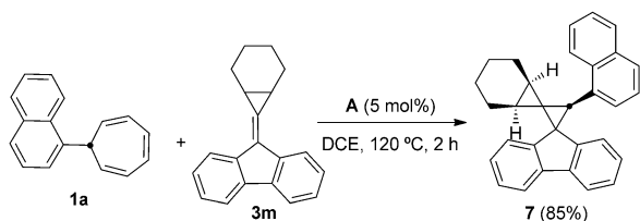
Scheme 3. Probing the mechanism of the formal (4+1) cycloaddition.
