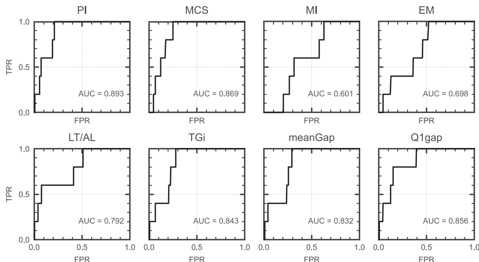
FIGURE 4 ROC curves for each evaluated metric, including their corresponding AUC for each curve. AUC, area under the curve; FPR, false positive rates; ROC, receiver operating characteristic; TPR, true positive rates.
