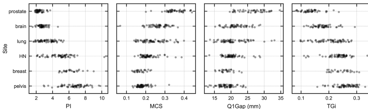
FIGURE 6 Complexity metrics as a function of the treatment site.
