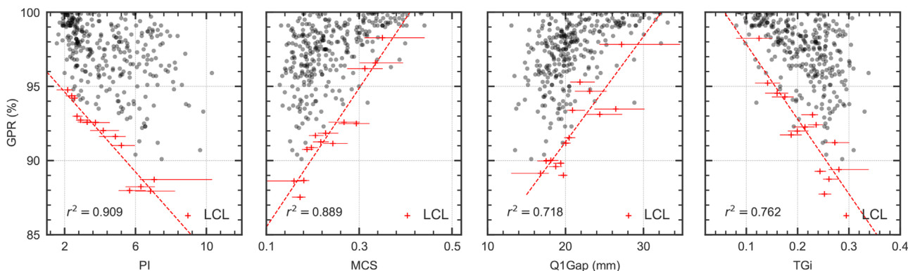
FIGURE 7 GPR results and LCL values relative to plan complexity. Circles represent GPR results. Red crosses indicate LCLs for similar complexity plans, positioned at each group’s median complexity, with the dashed line indicating the linear fit. GPR, gamma passing rate; LCL, lower control limit.
