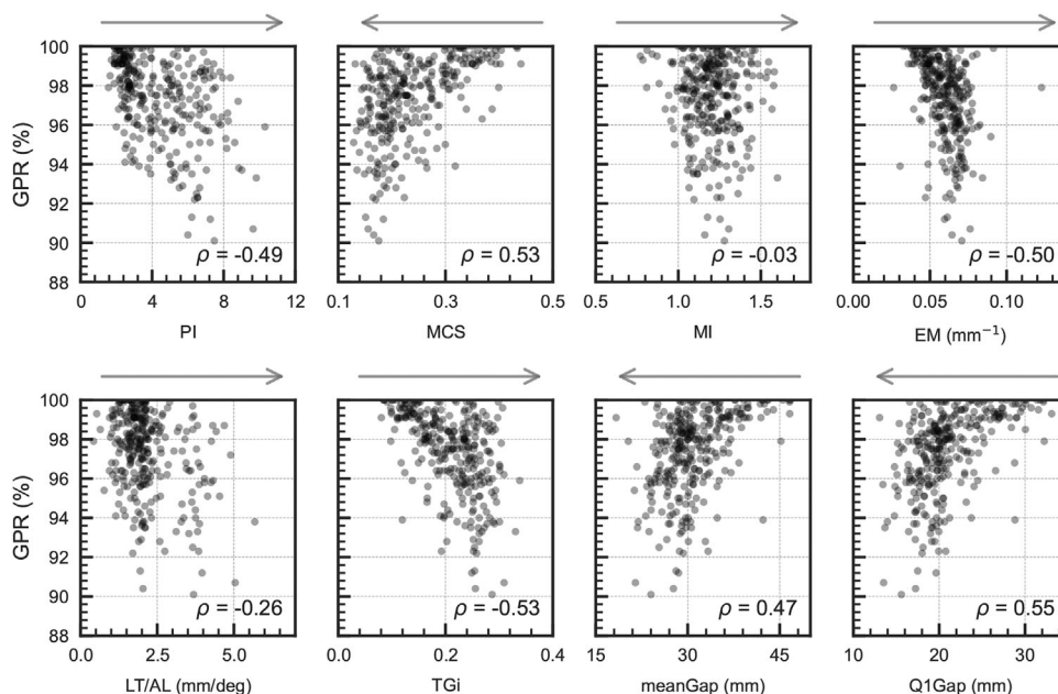
FIGURE 3 Relationship between GPR and evaluated plan complexity metrics with their corresponding Spearman's correlation coefficient r . Arrows indicate the direction of increasing plan complexity for each metric. Note that plan complexity increases with the score for PI, MI, EM, LT/AL, and TG i , while for MCS, meanGap, and Q1Gap plan complexity decreases with the metric's value. EM, edge metric; GPR, gamma passing rates; LT/AL, leaf travel divided by the arc length; MI, modulation index; meanGap, mean MLC gap; PI, plan irregularity; TG i , tongue-and-groove index.
