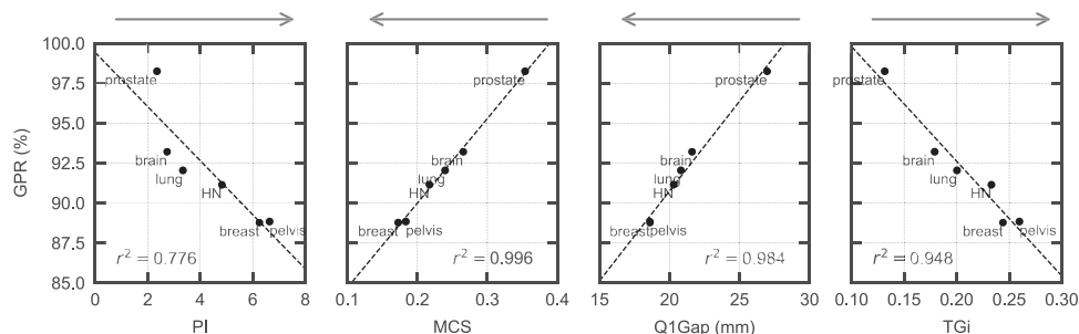
FIGURE 5 Relationship between LCL values and average complexity metrics for each treatment site, including a linear fit with its correlation coefficient r^2 . Arrows indicate the direction of increasing plan complexity for each metric. LCL, lower control limit.
