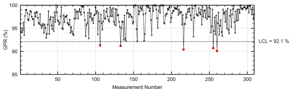
FIGURE 2 I-chart for the pre-treatment verification process, with symbols representing time-ordered results. Black symbols indicate in-control results, while red symbols show out-of-control data points. GPR, gamma passing rate; LCL, lower control limit.
